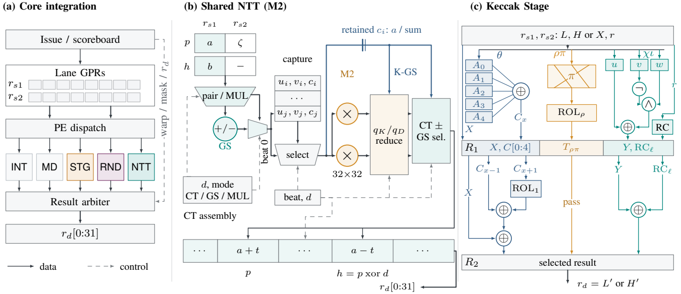
Fig. 2. Core integration and collective datapaths. (a) Dedicated PEs share operand dispatch and result arbitration with INT and multiply/divide. (b) K/D share preparation, capture, M2, reduction, and indexed assembly. Beat zero bypasses capture; c_i retains a or the GS sum. CT writes are shown with t = \text{Mont}_Q(b\zeta) . (c) Three alternative Stage paths cross R_1/R_2 . A_i = A[x, i] combines L/H ; u, v, w are row-neighbor halves; RC_l is zero except at lane zero.
