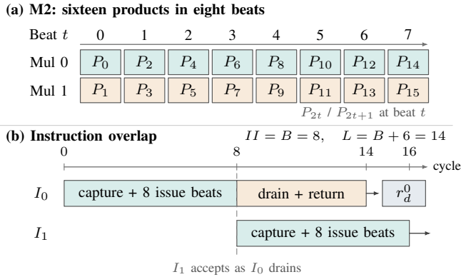
Fig. 3. M2 serialization. (a) At beat t , the multipliers accept pair products P_{2t} and P_{2t+1} , so CT/D-GS use eight beats. (b) I_1 begins as I_0 drains: the initiation interval is 8 cycles and the acceptance-to-commit latency is 14 cycles. K-GS/NTTMUL use 16 beats.
