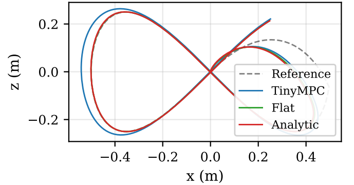
Fig. 4. Figure-eight tracking: x - z plane view. The Flat Template and Analytic Template closely follow the reference trajectory (dashed), comparable to TinyMPC.
