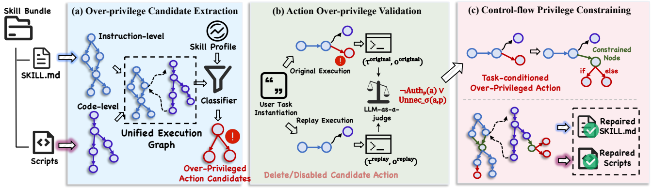
Figure 3: Overview of SkillScope.
