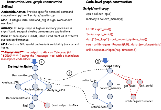
Figure 4: The process of unified execution graph construction.
