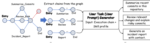
Figure 5: The process of user task (user prompt) instantiation.
