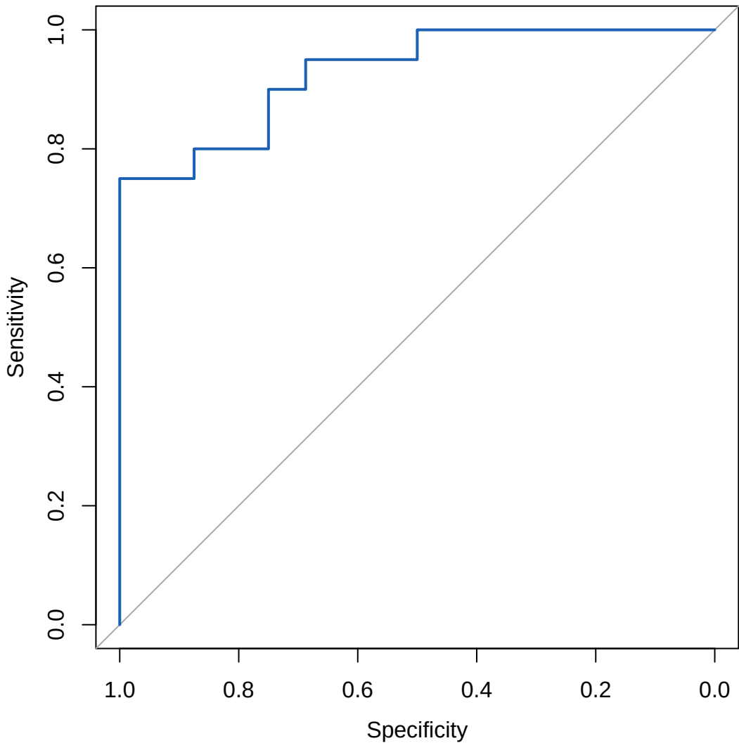
ROC curve for BKP (AUC = 0.928)
