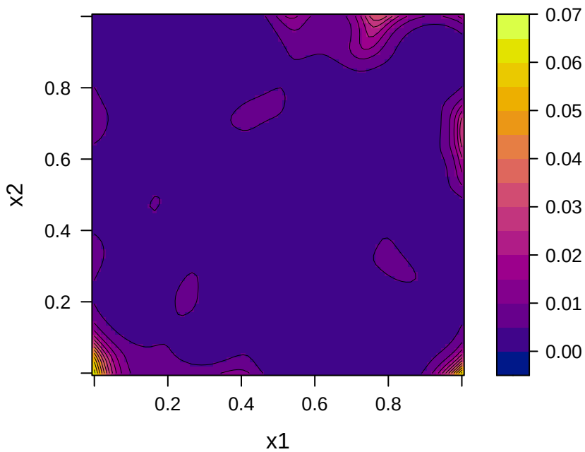
Predictive Variance
