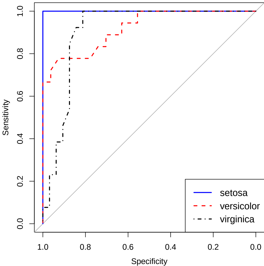
One-vs-Rest ROC curve for BKP (AUC =0.944)
