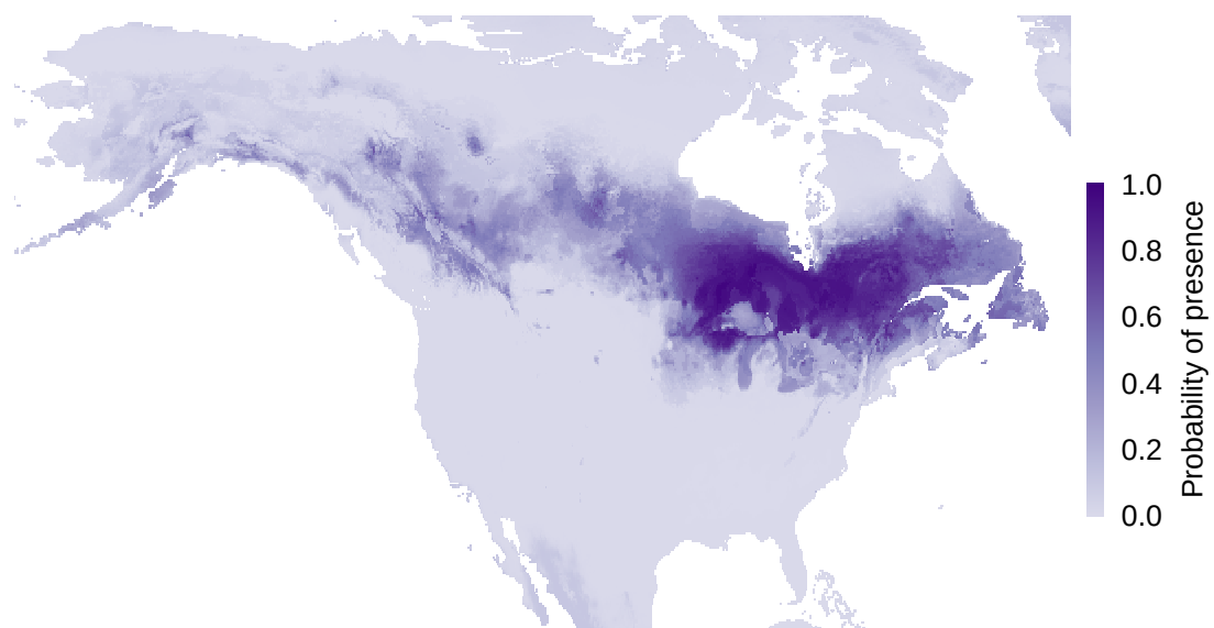
(c) TwinBKP – Predicted distribution
