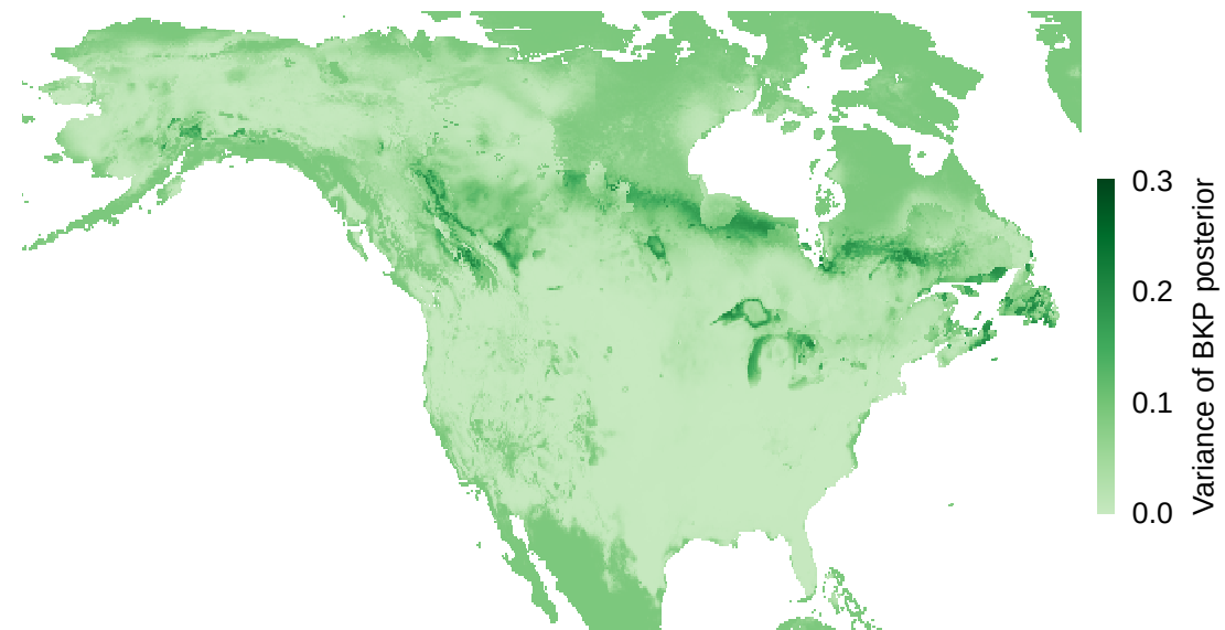
(b) BKP – Prediction uncertainty
