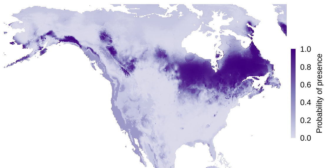
(e) LGP – Predicted distribution
