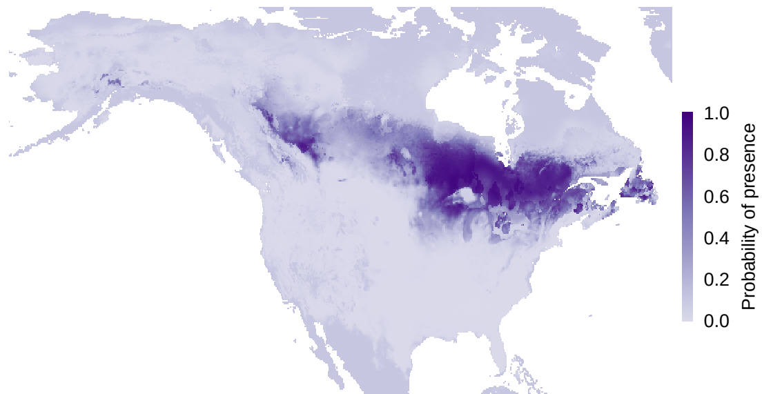
(a) BKP – Predicted distribution
