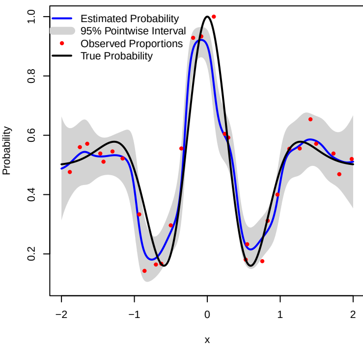
(c) BKP-ESS, n=30
