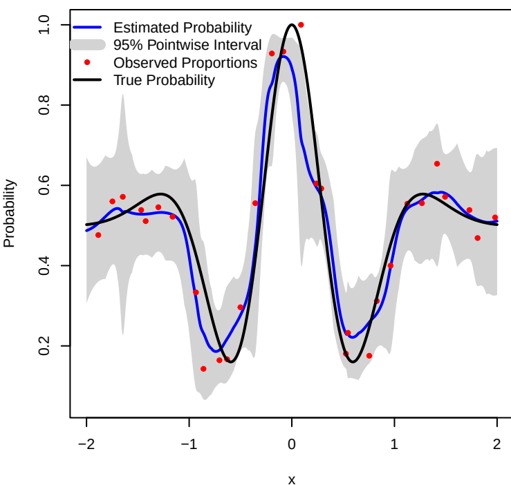
(e) LGP, n=30
