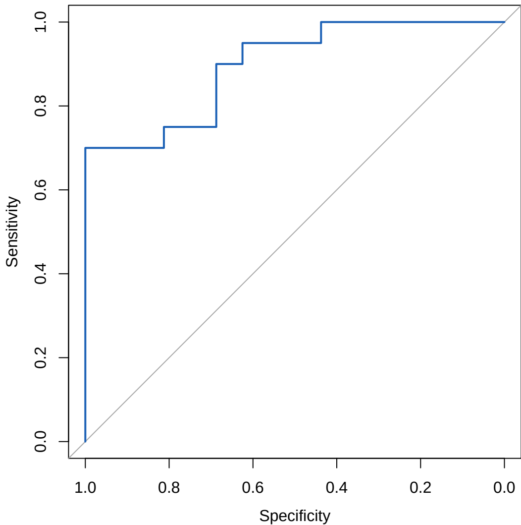
ROC curve for LGP (AUC = 0.897)
