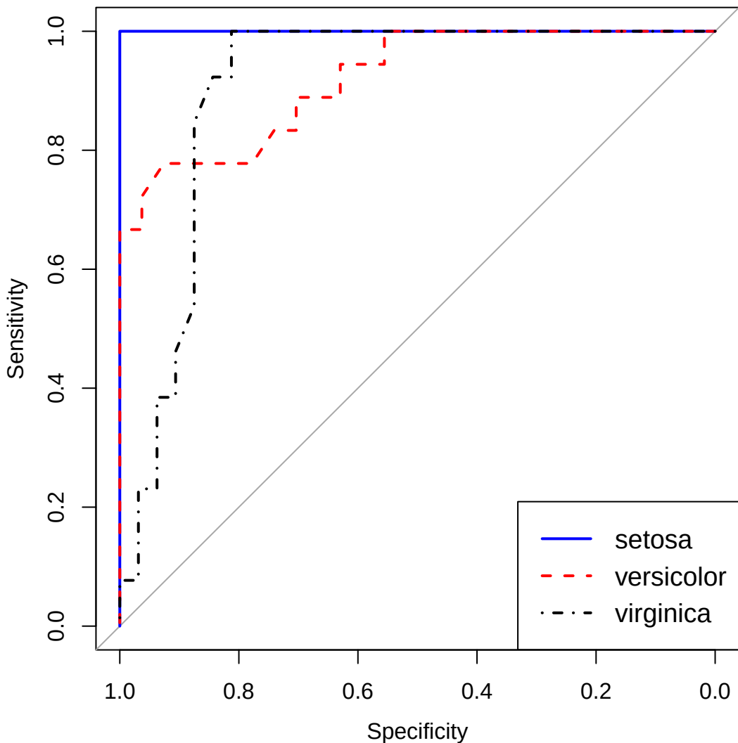
One-vs-Rest ROC curve for DKP (AUC =0.944)
