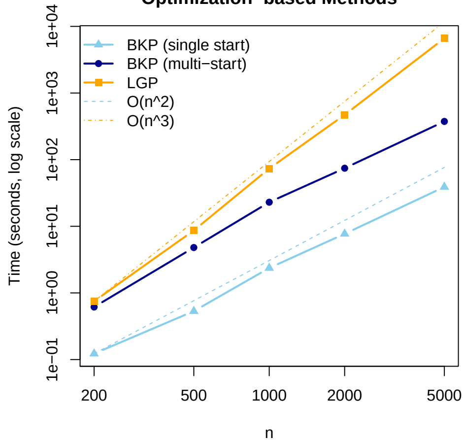
Optimization-based Methods
