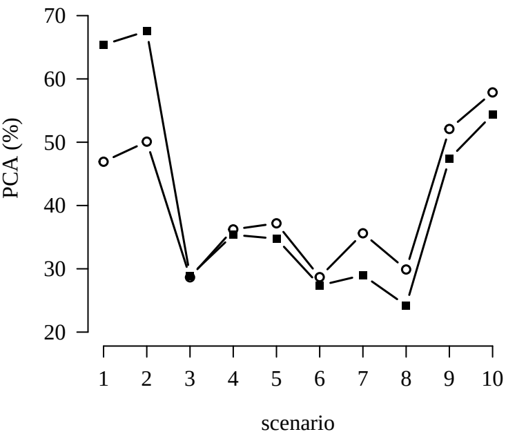
(c) PCA under \phi = 0.2
