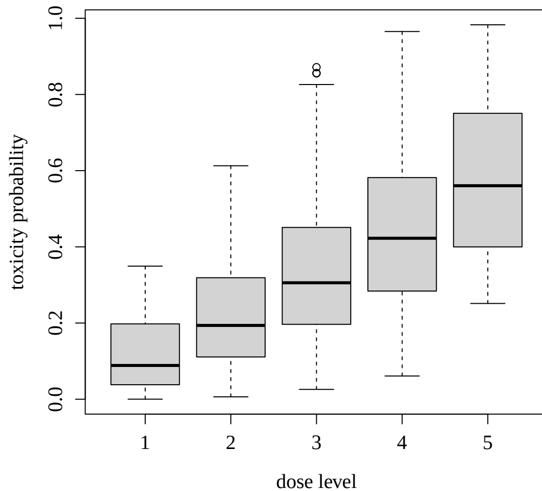
(b) toxicity distribution
