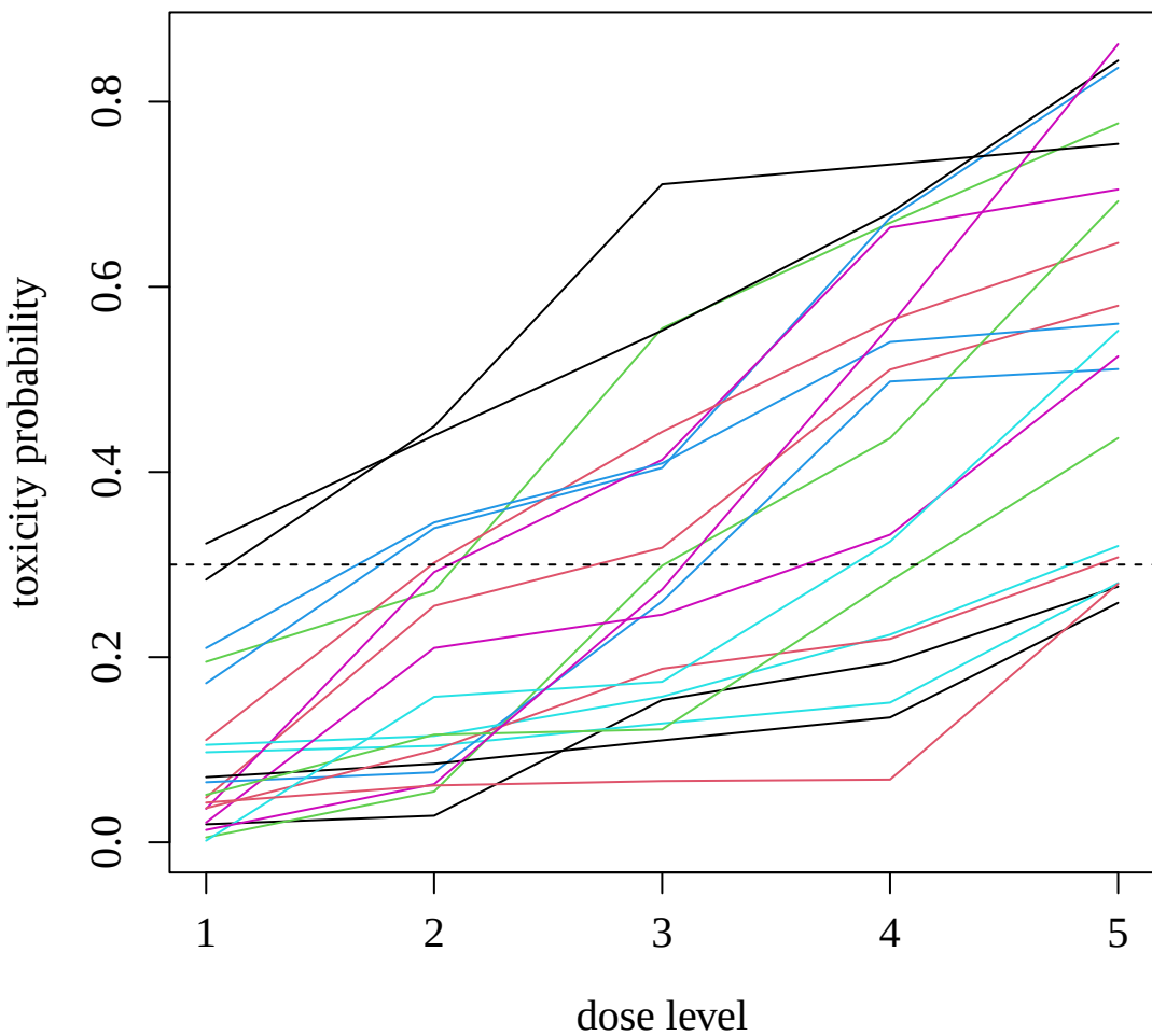
(a) dose-toxicity curves
