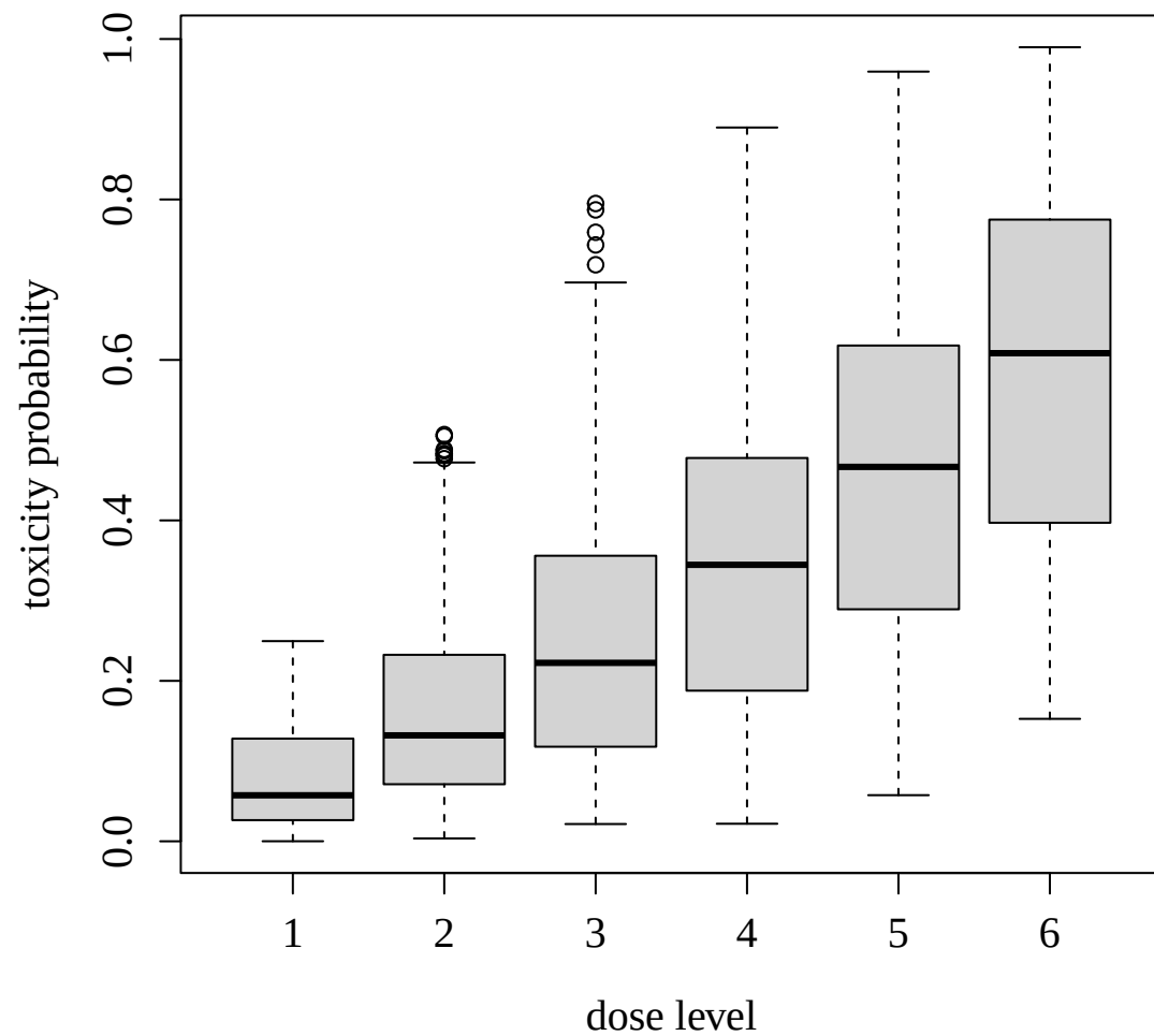
(b) toxicity distribution
