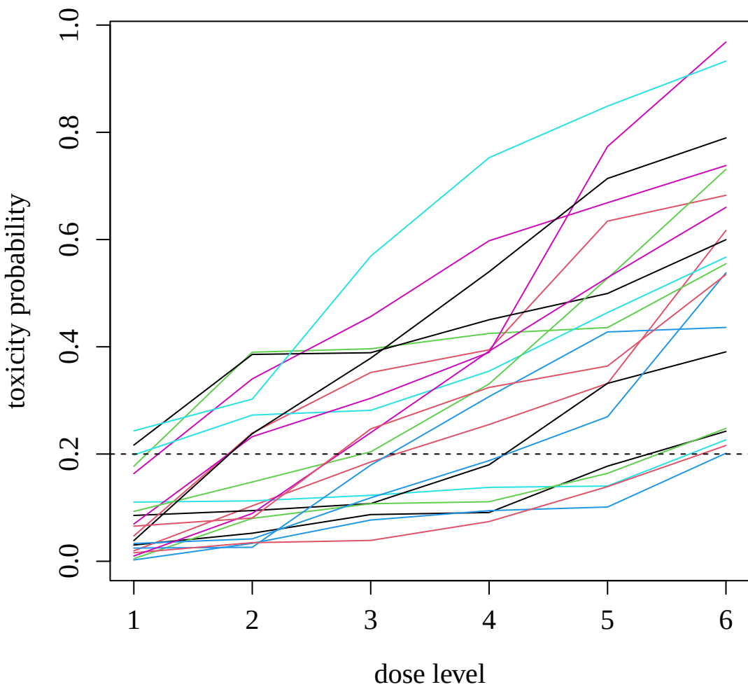
(a) dose-toxicity curves
