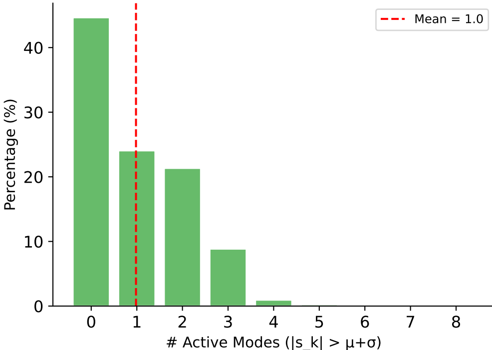
(C) Sparsity: Modes per Sample (threshold=0.418)
