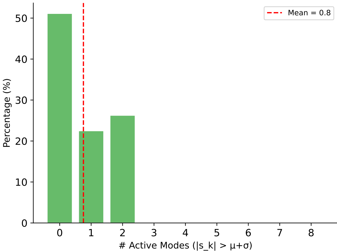
(C) Sparsity: Modes per Sample (threshold=0.605)
