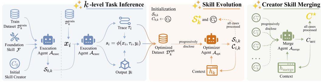
Figure 3: Overview of our evolution pipeline. The execution agent \mathcal{A}_{\text{exec}} first performs task inference to generate initial category-level composition skills S_{0,k} and collect execution traces \tau , outputs y , and evaluation feedback s_i . The optimizer agent \mathcal{A}_{\text{opt}} then progressively refines composition skills and creator skills with feedback to obtain S_k^* and C_k^* . Finally, the merge agent \mathcal{A}_{\text{merge}} integrates multiple creator skills into a single C^* .
