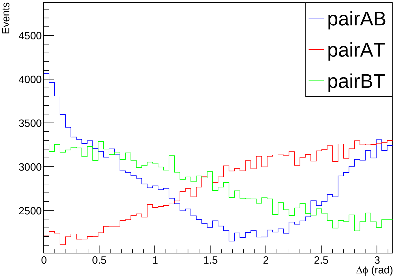
Delta Phi Between Momentum Vectors - Mass Difference Selection
