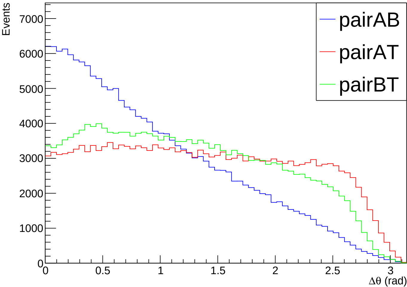
Delta Theta Between Momentum Vectors - Mass Difference Selection
