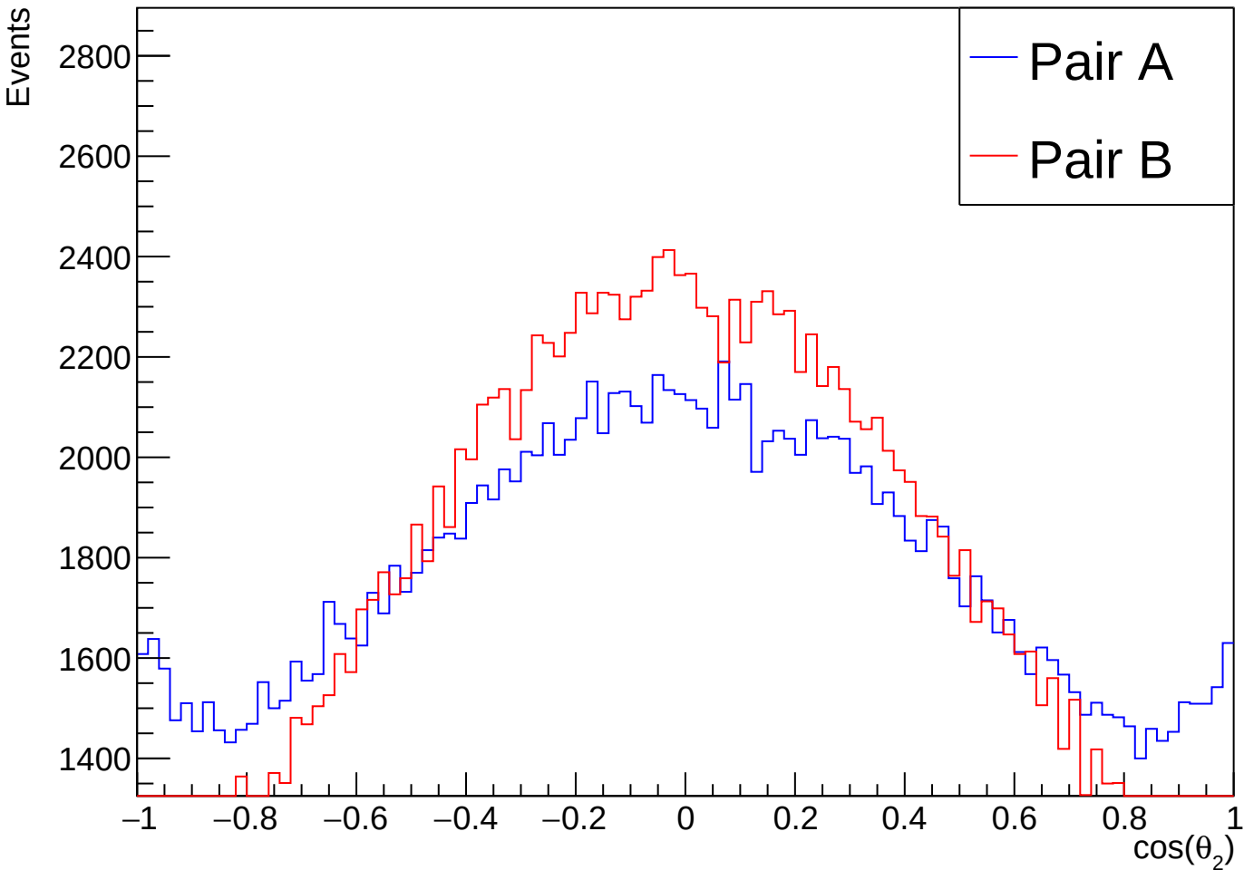
\cos(\theta_2) Pion Momentum vs Z-axis in Pair Rest Frame - Mass Difference Selection
