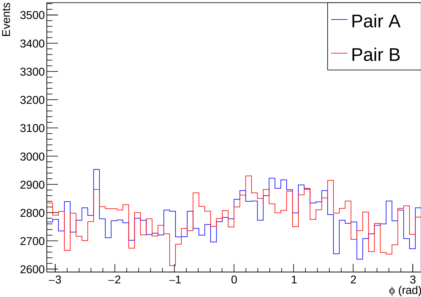
Phi Angles of Relative Momentum Vectors - Mass Difference Selection
