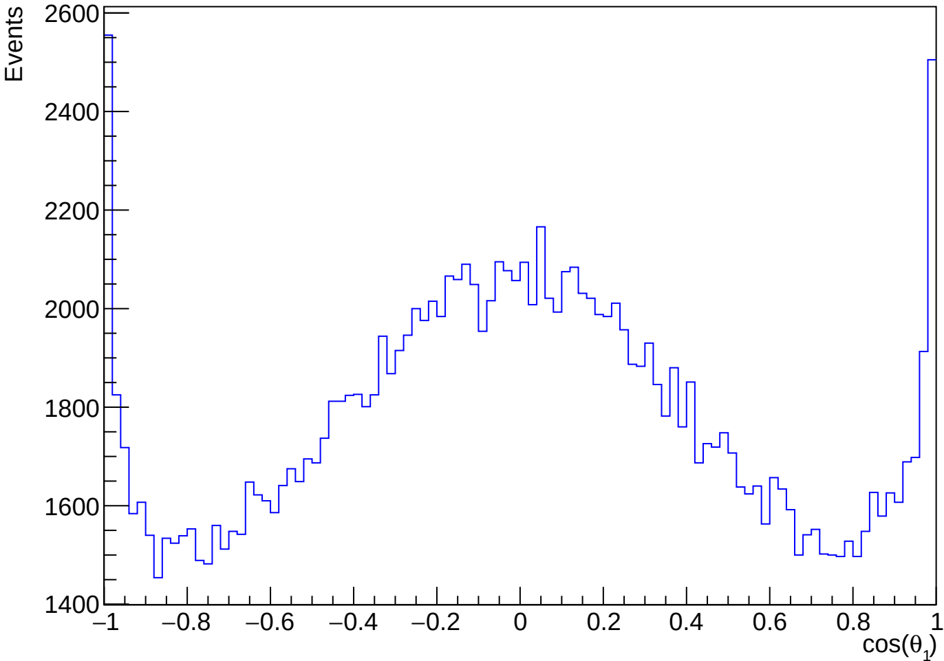
\cos(\theta_1) Pair Momentum vs Z-axis in 4\pi Rest Frame - Mass Difference Selection
