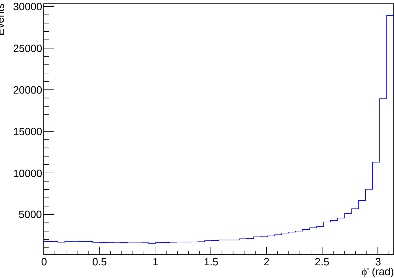
Phi Prime - Angle Between Two Pair pT Vectors - Mass Difference Selection
