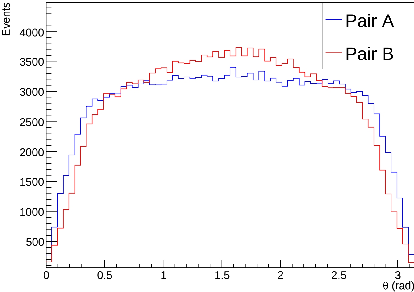
Theta Angles of Relative Momentum Vectors - Mass Difference Selection
