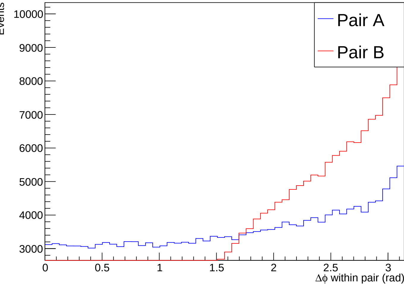
Phi Difference Within Pairs - Mass Difference Selection
