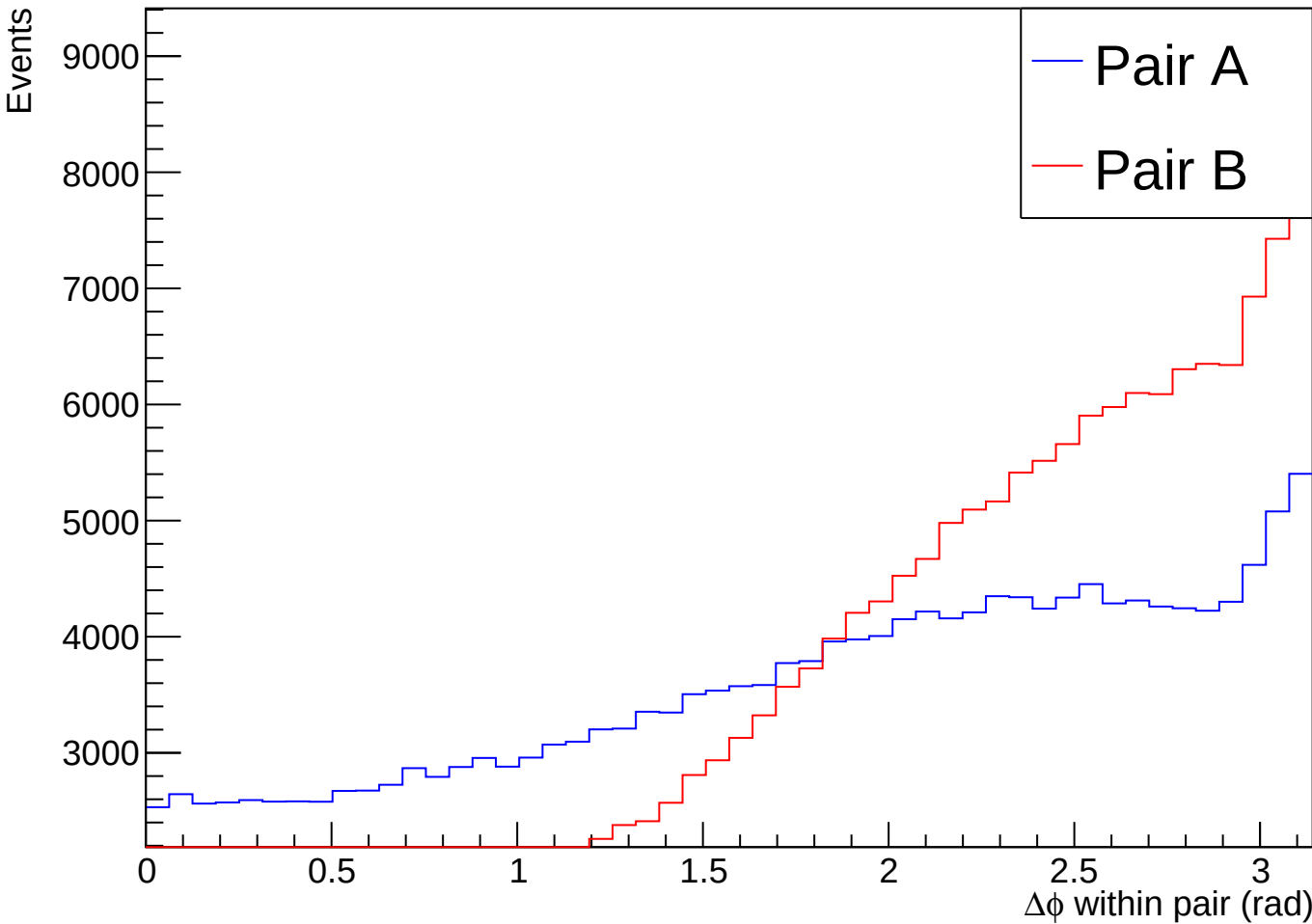
Phi Difference Within Pairs - pT Difference Selection
