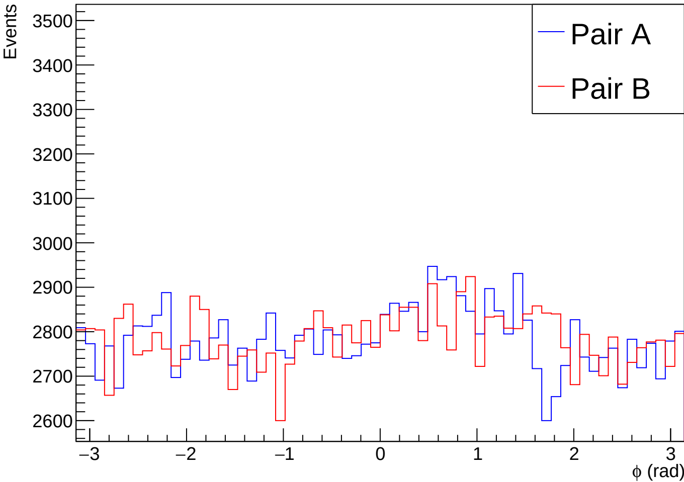
Phi Angles of Relative Momentum Vectors - pT Difference Selection
