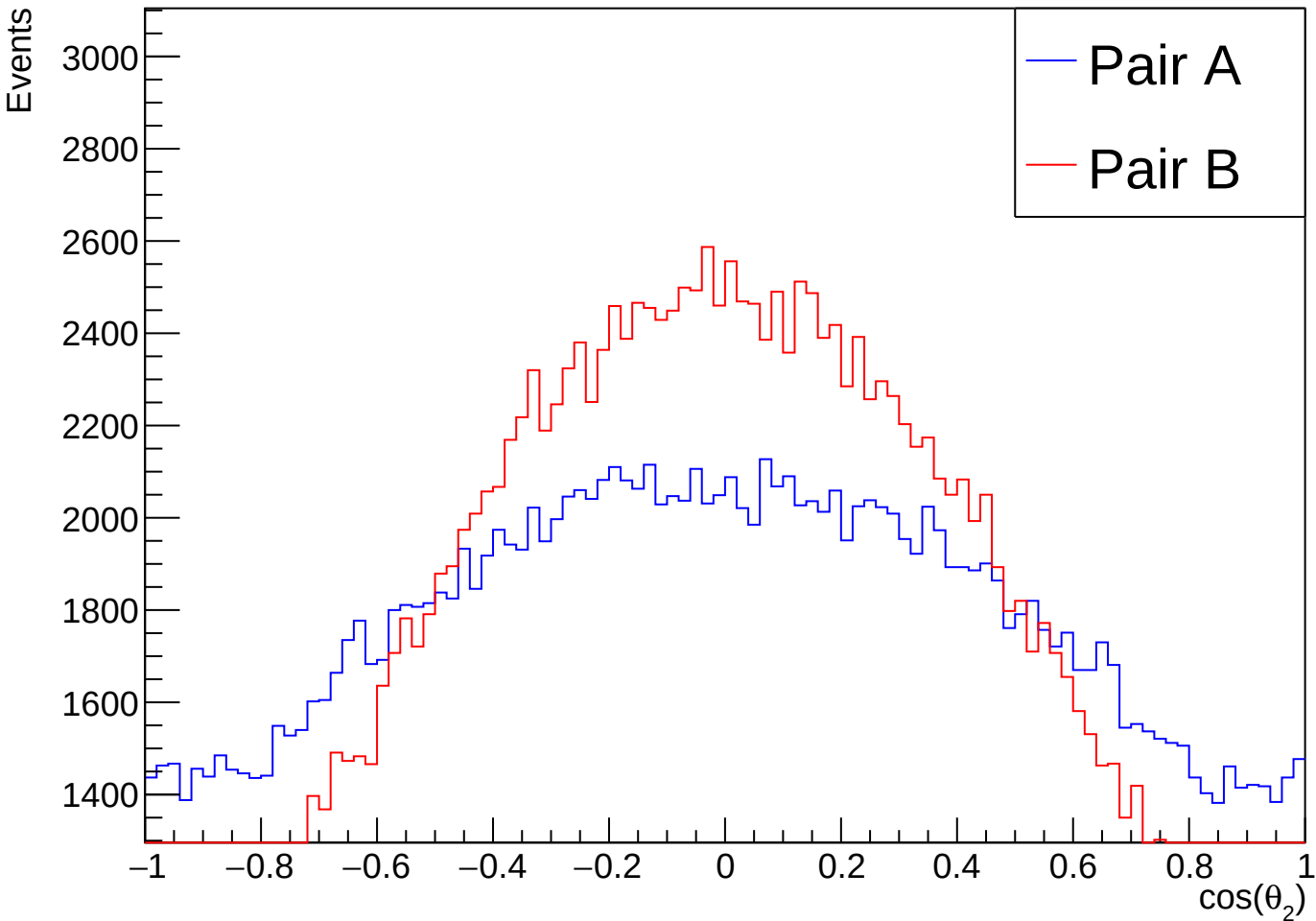
\cos(\theta_2) Pion Momentum vs Z-axis in Pair Rest Frame - pT Difference Selection
