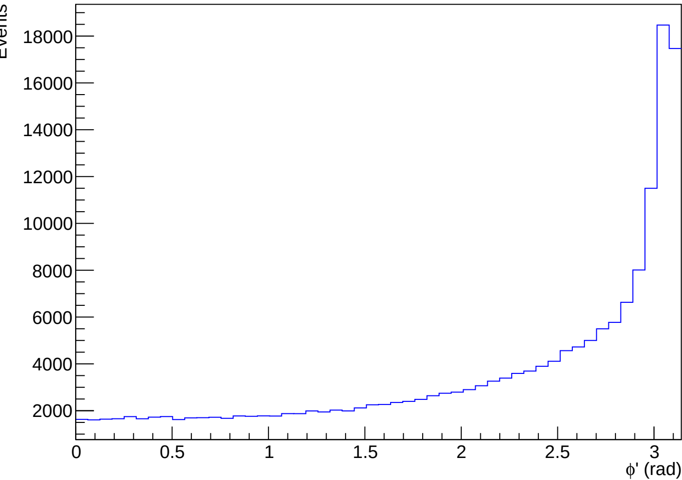
Phi Prime - Angle Between Two Pair pT Vectors - pT Difference Selection
