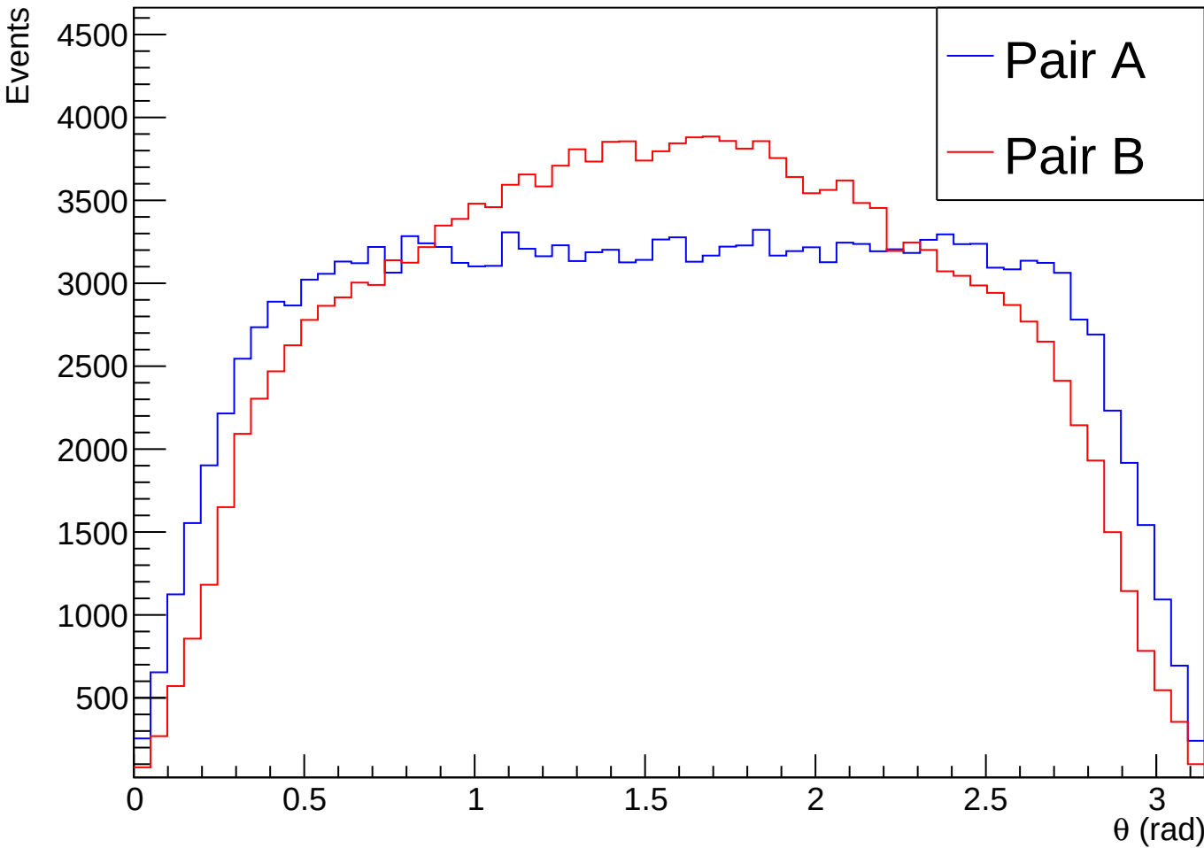
Theta Angles of Relative Momentum Vectors - pT Difference Selection
