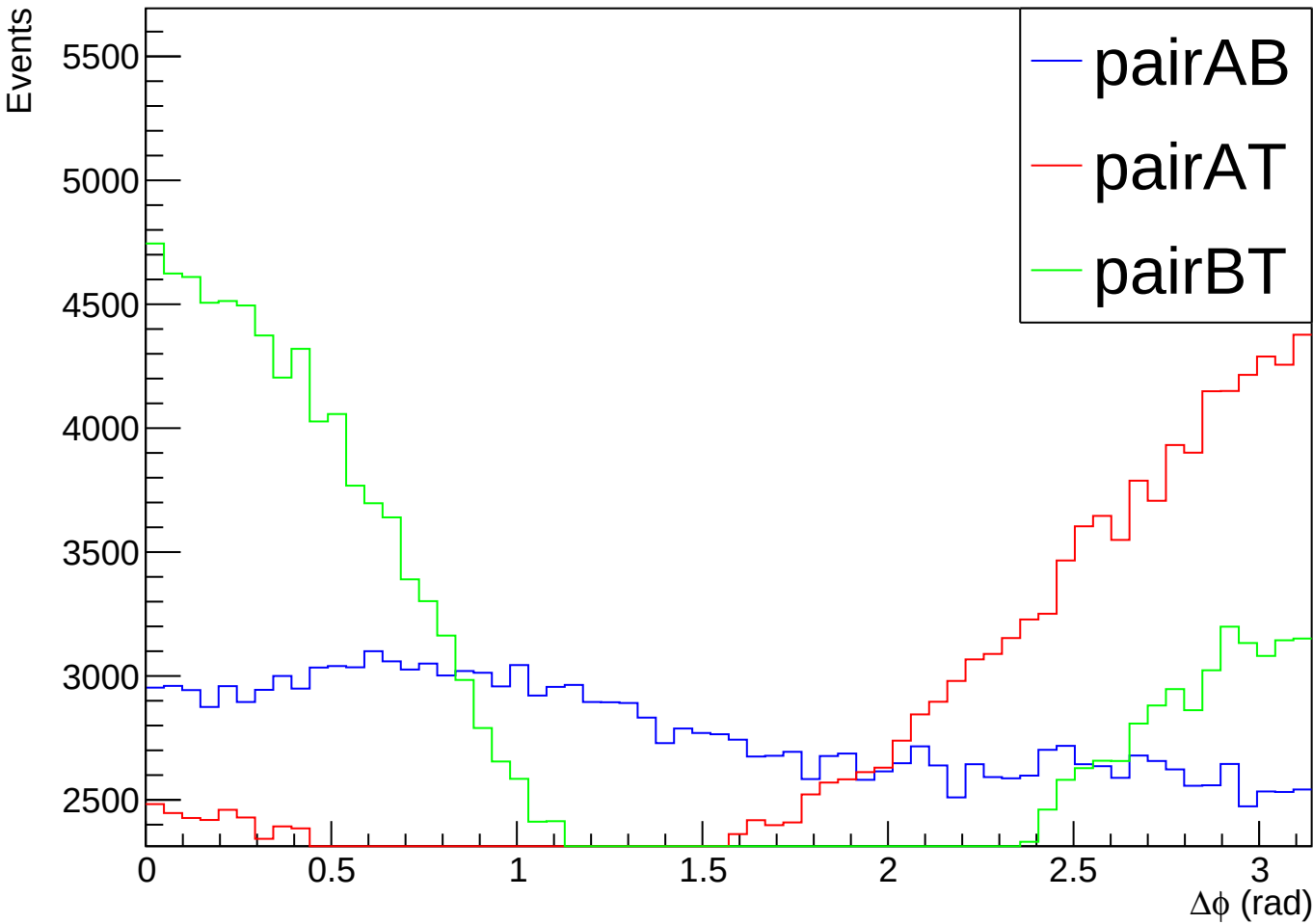
Delta Phi Between Momentum Vectors - pT Difference Selection
