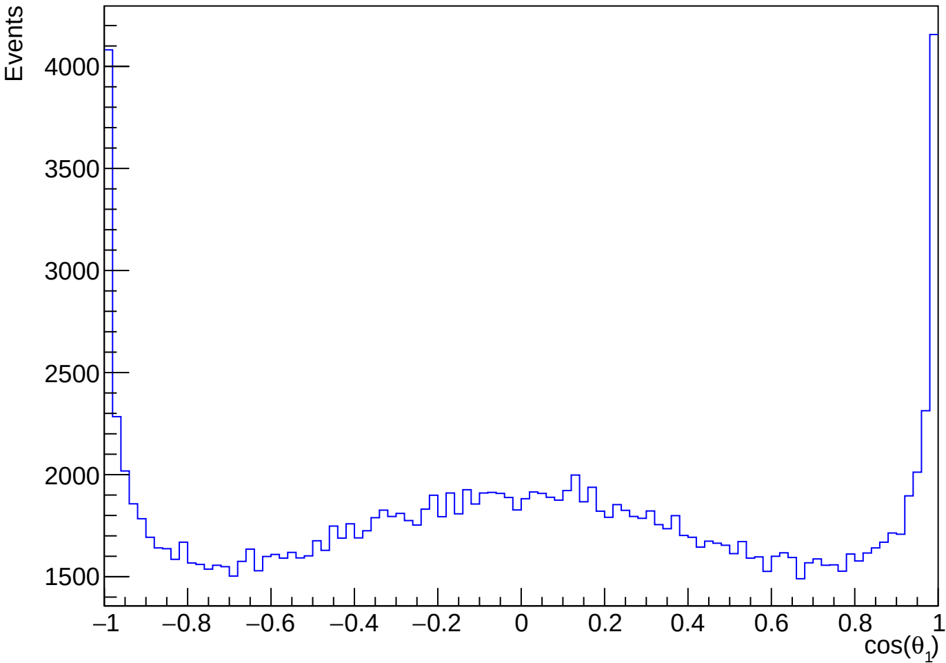
\cos(\theta_1) Pair Momentum vs Z-axis in 4\pi Rest Frame - pT Difference Selection
