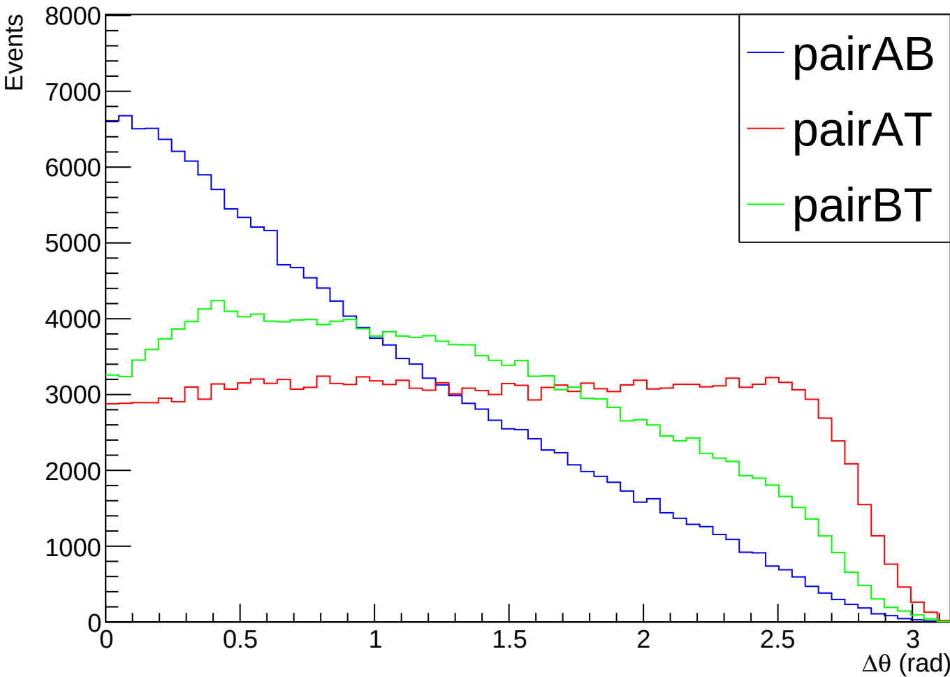
Delta Theta Between Momentum Vectors - pT Difference Selection
