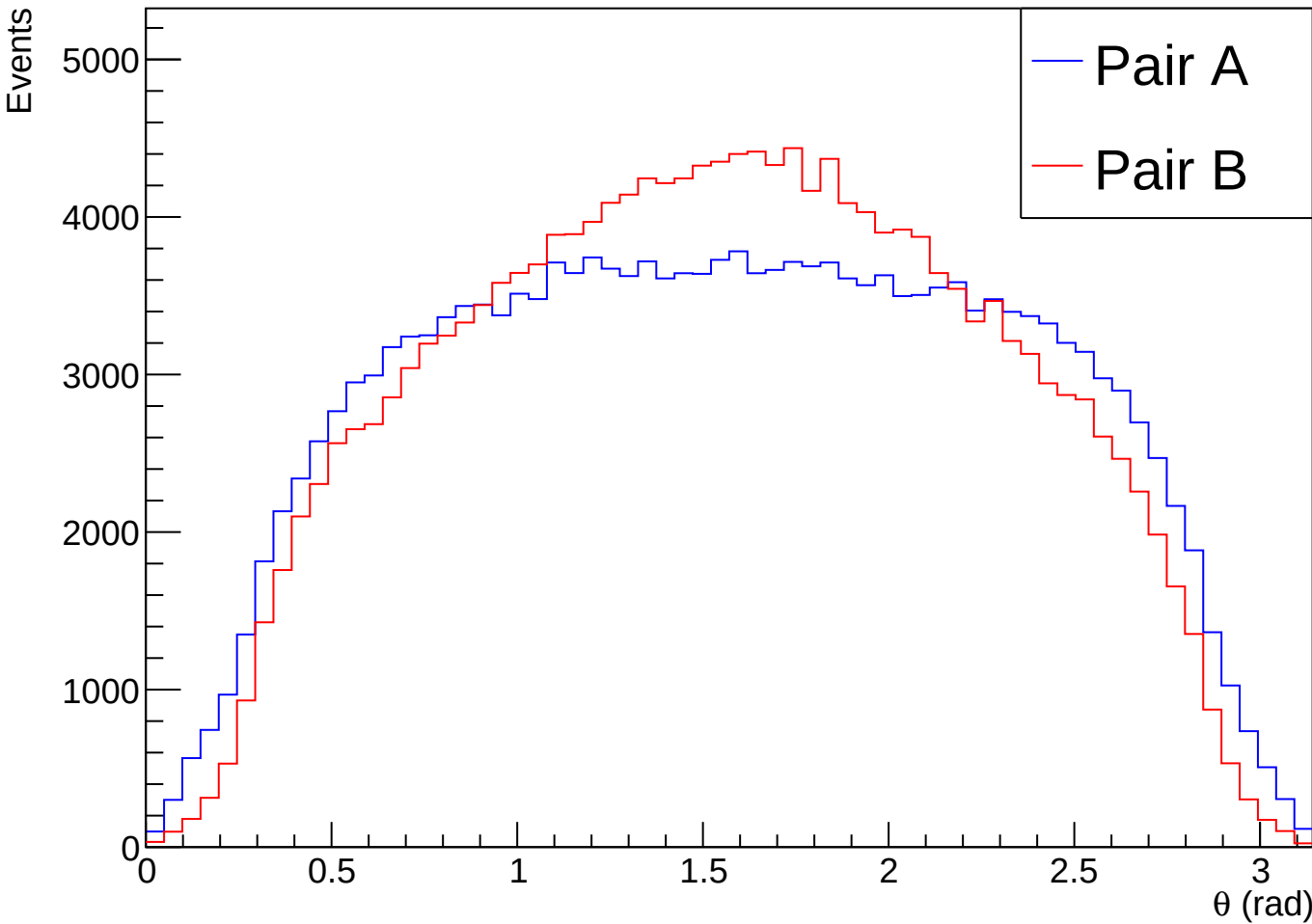
Theta Angles of Relative Momentum Vectors - pT Sum Selection
