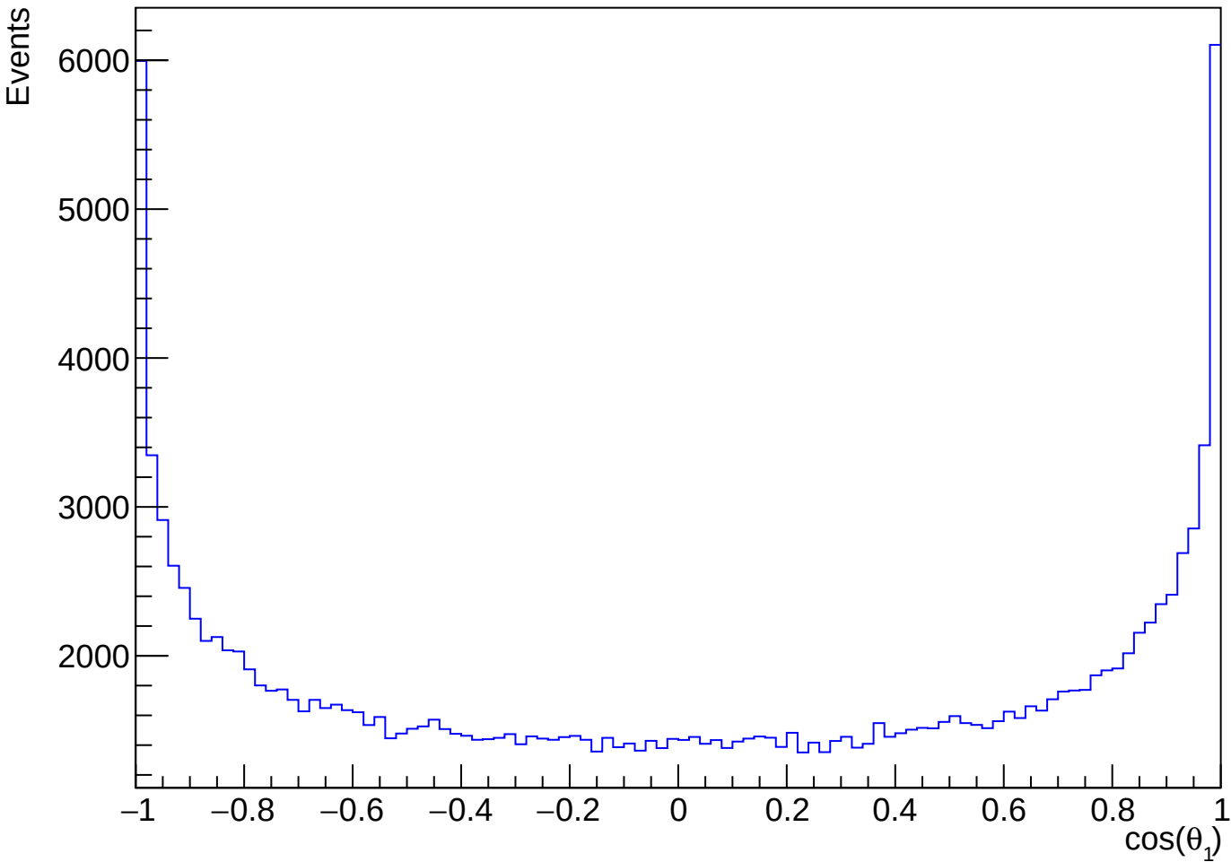
\cos(\theta_1) Pair Momentum vs Z-axis in 4\pi Rest Frame - pT Sum Selection
