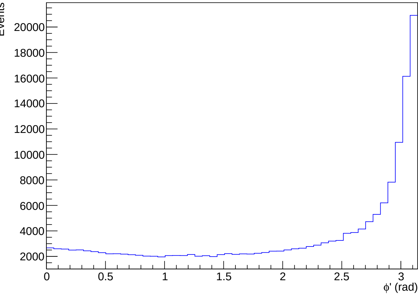
Phi Prime - Angle Between Two Pair pT Vectors - pT Sum Selection
