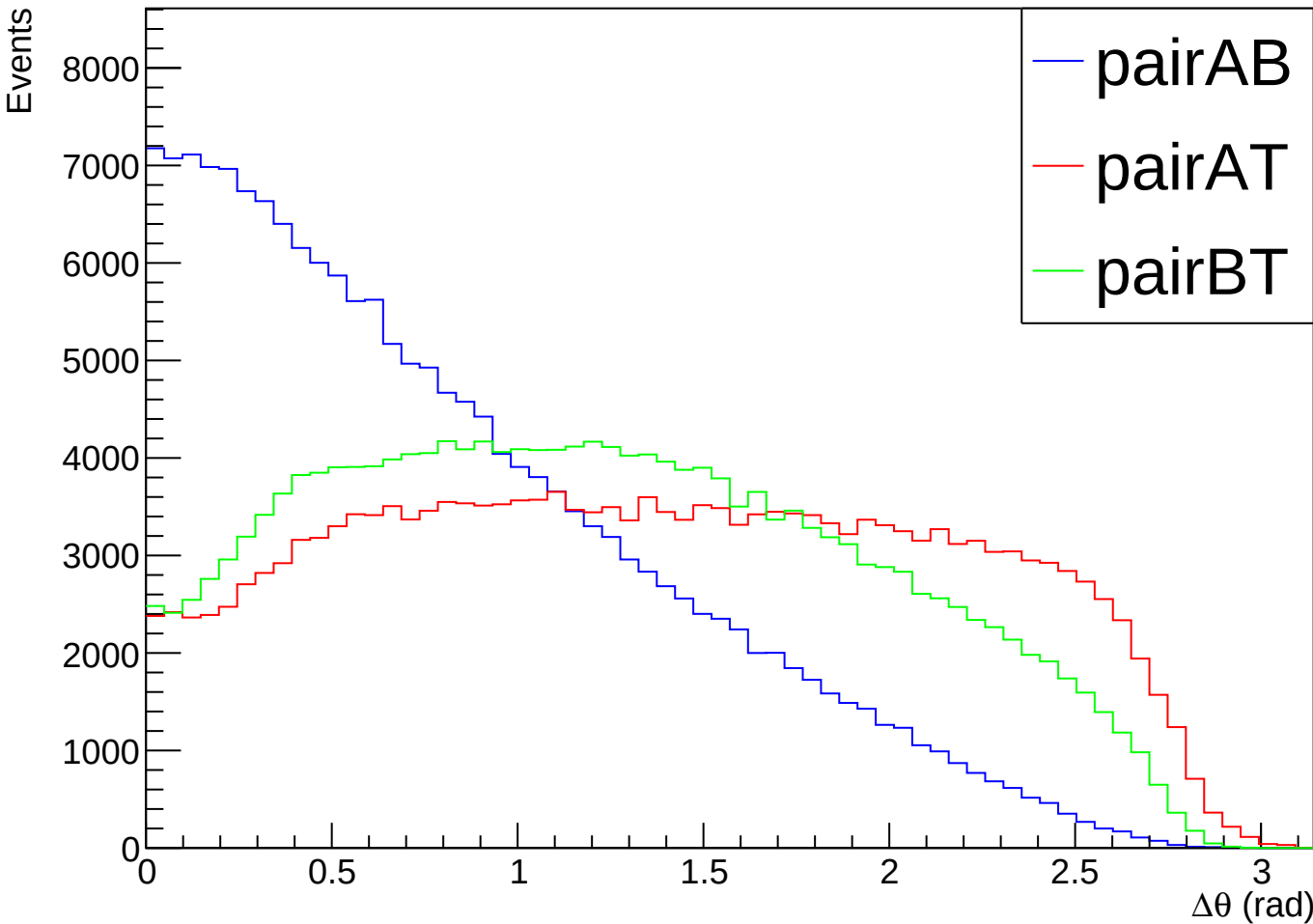
Delta Theta Between Momentum Vectors - pT Sum Selection
