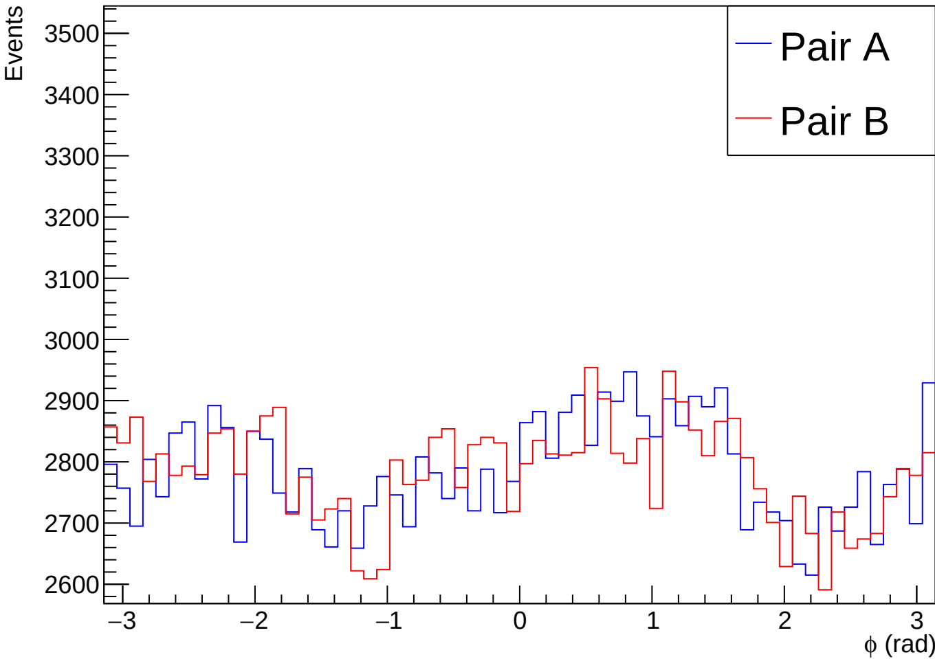
Phi Angles of Relative Momentum Vectors - pT Sum Selection
