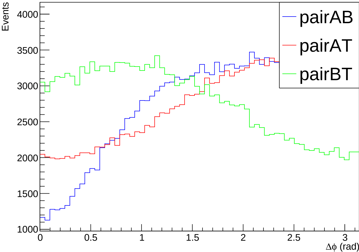
Delta Phi Between Momentum Vectors - pT Sum Selection
