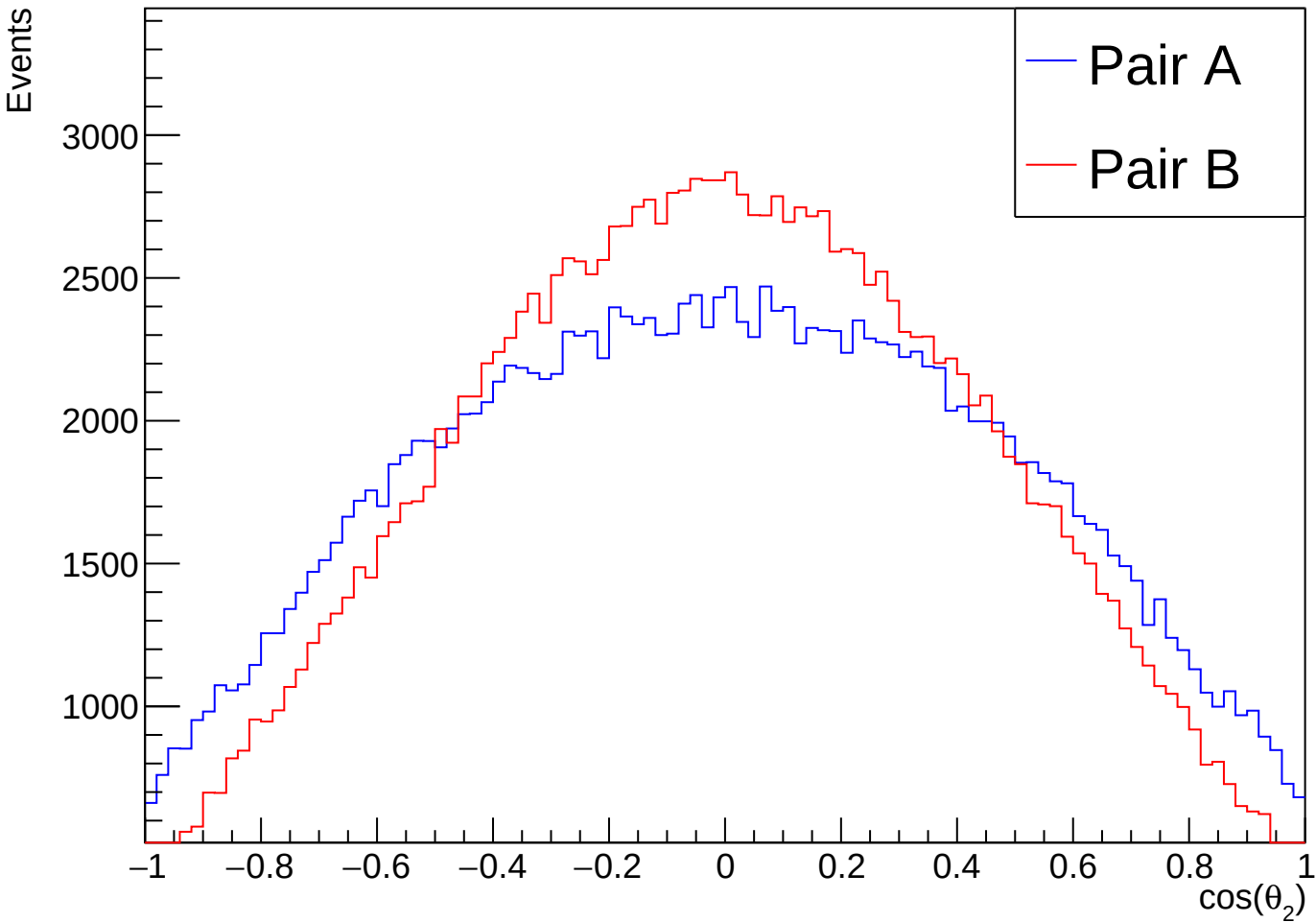
\cos(\theta_2) Pion Momentum vs Z-axis in Pair Rest Frame - pT Sum Selection
