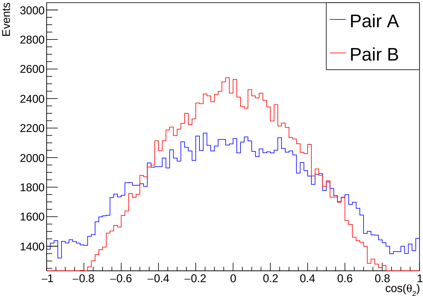
\cos(\theta_2) Pion Momentum vs Z-axis in Pair Rest Frame - Random Selection
