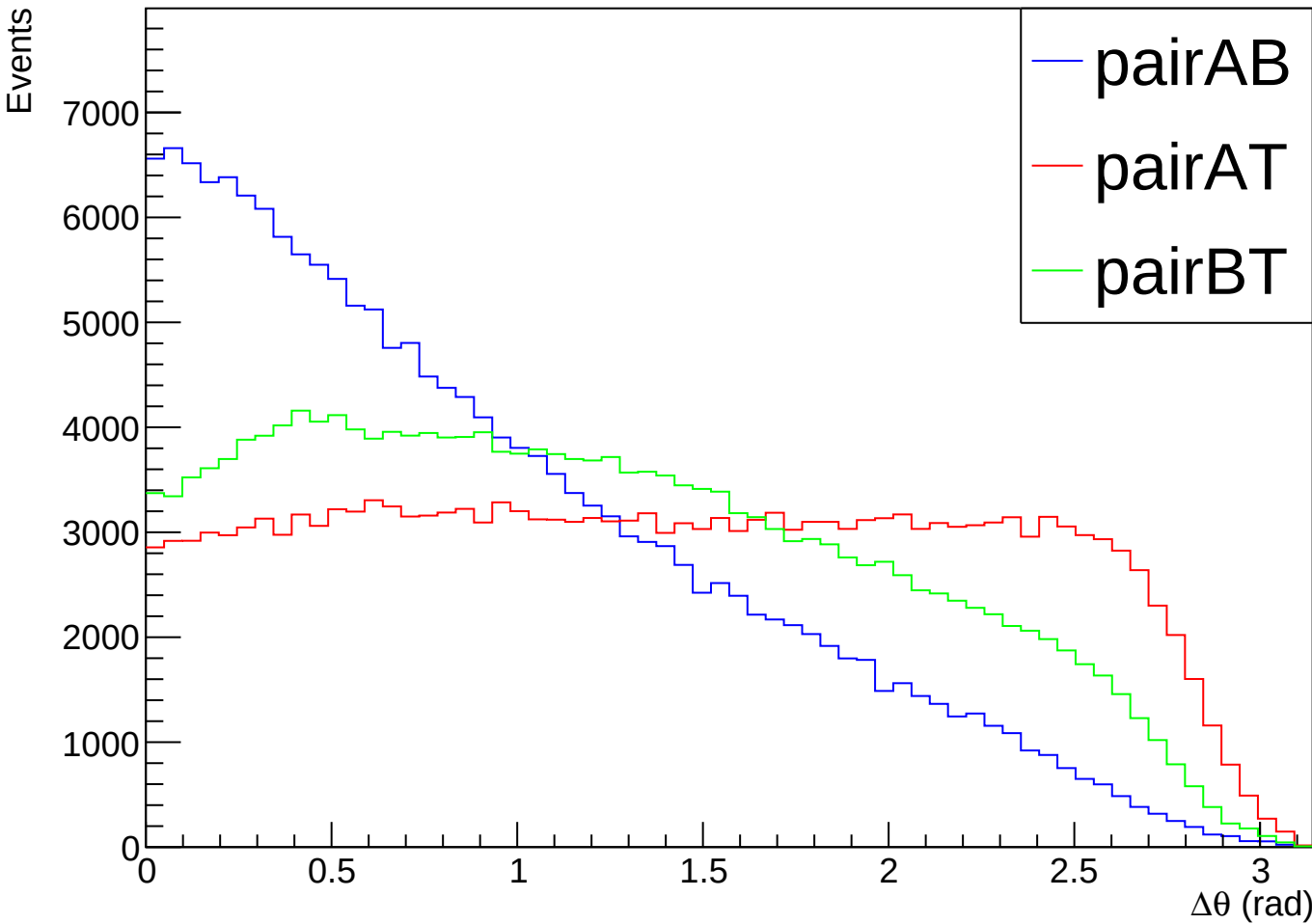
Delta Theta Between Momentum Vectors - Random Selection
