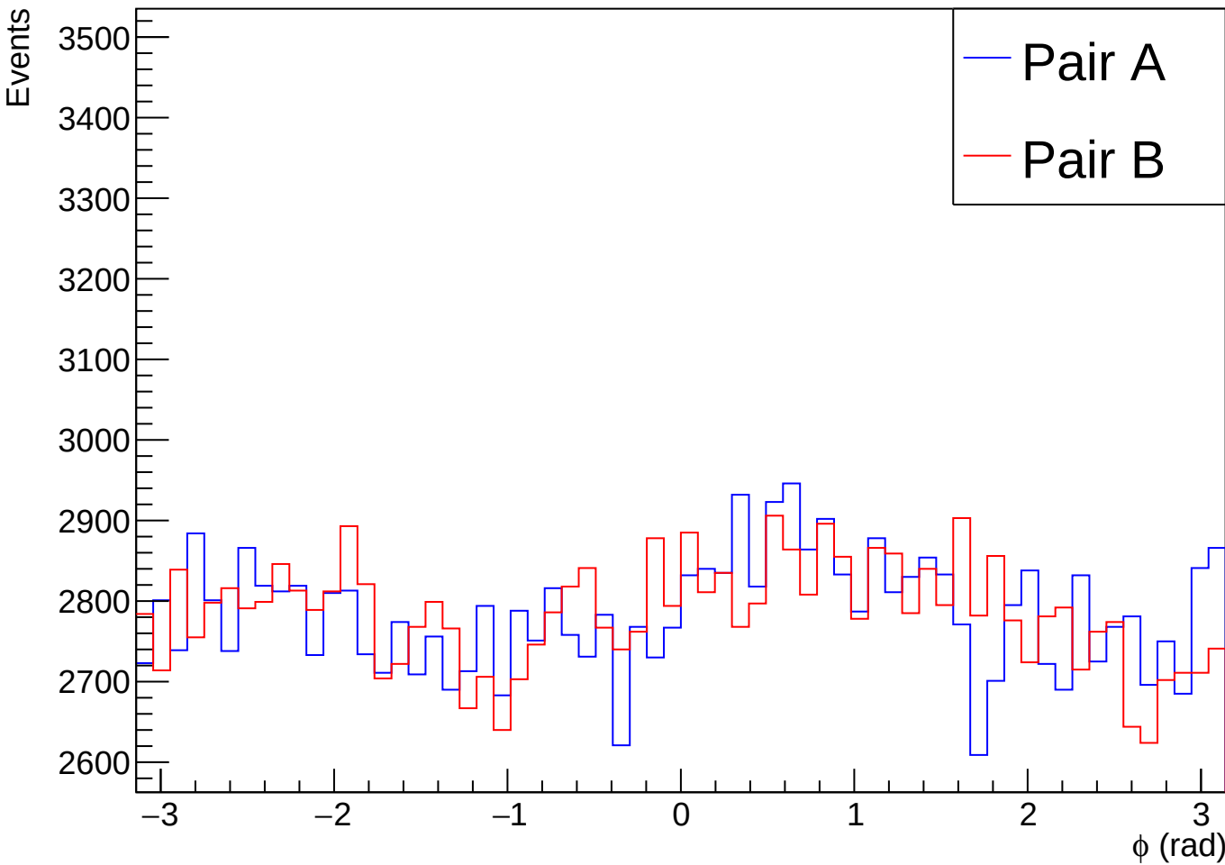
Phi Angles of Relative Momentum Vectors - Random Selection
