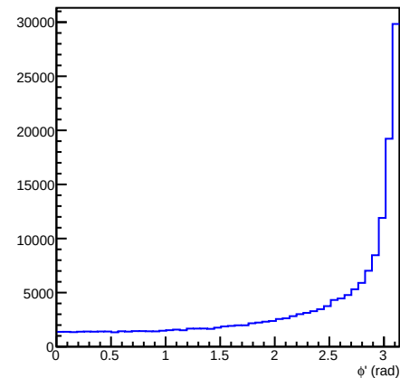
Phi Prime - Angle Between Pair pT
