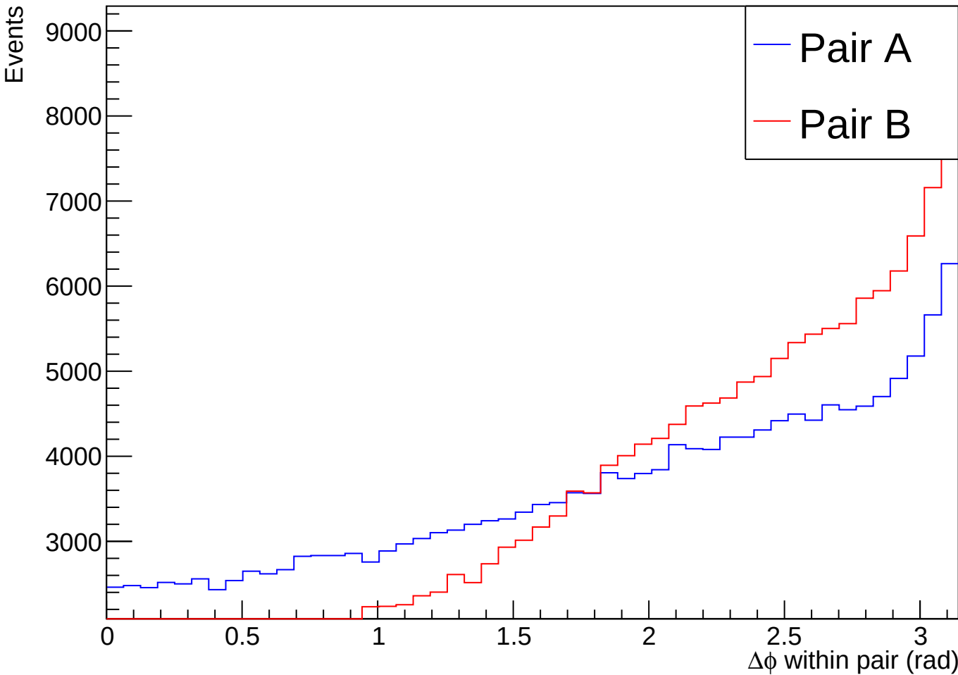
Phi Difference Within Pairs - Random Selection
