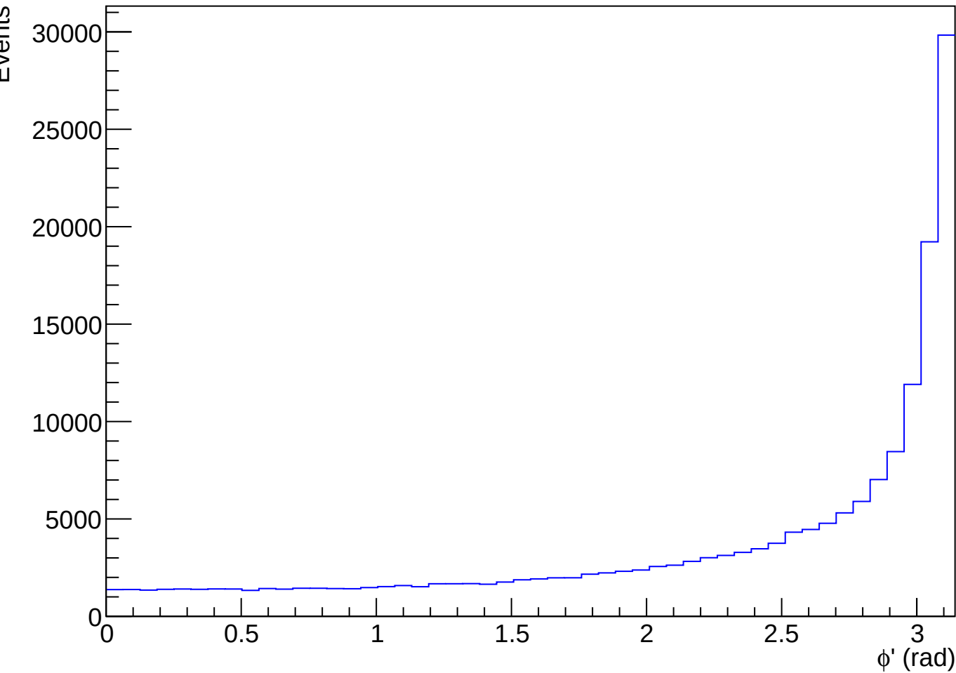
Phi Prime - Angle Between Two Pair pT Vectors - Random Selection
