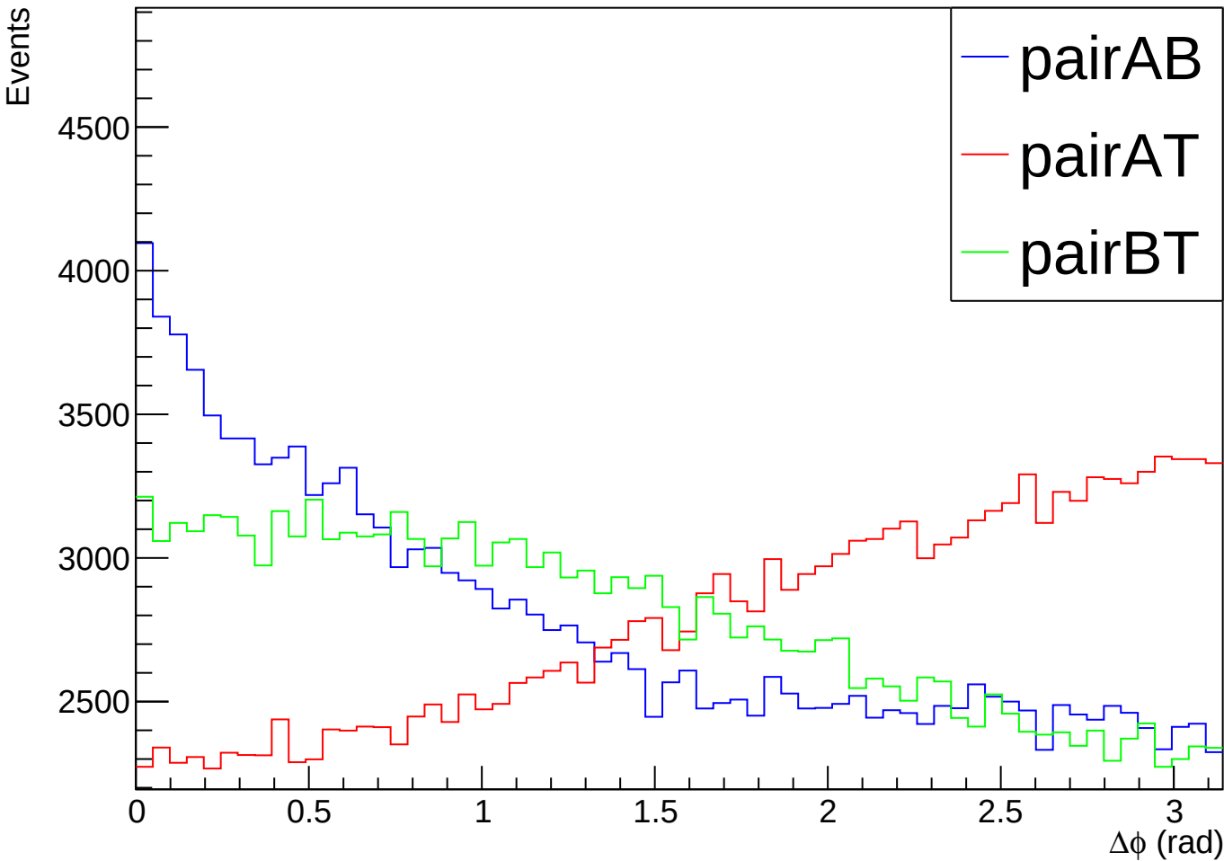
Delta Phi Between Momentum Vectors - Random Selection
