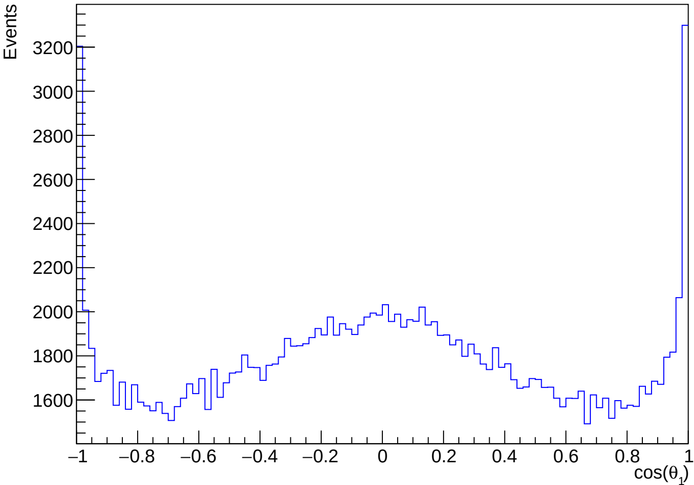
\cos(\theta_1) Pair Momentum vs Z-axis in 4\pi Rest Frame - Random Selection
