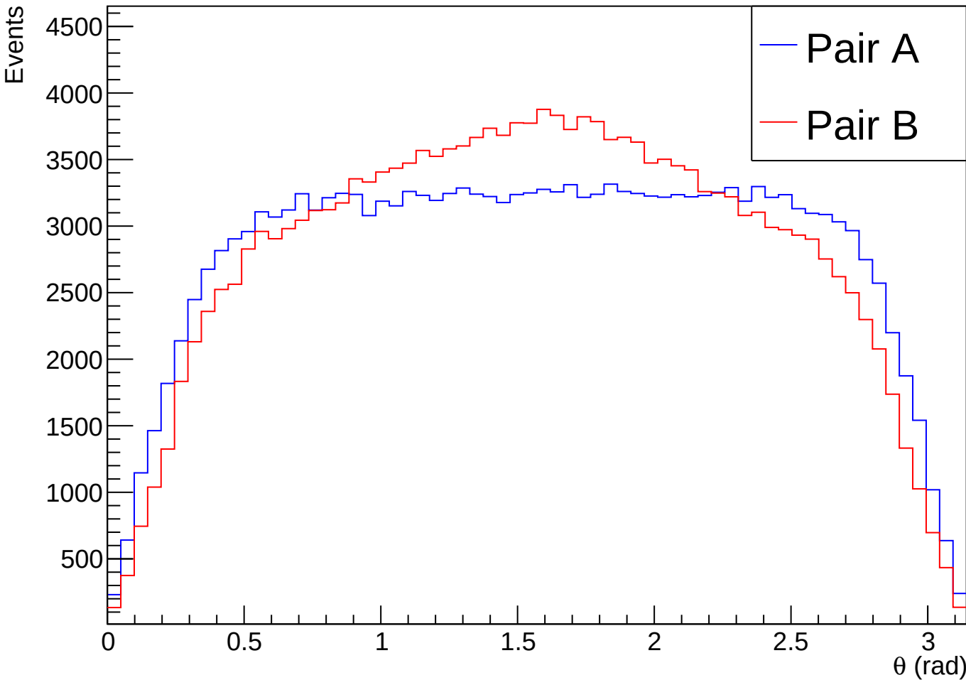
Theta Angles of Relative Momentum Vectors - Random Selection
