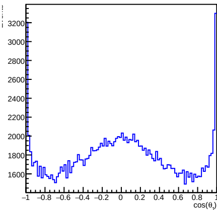
\cos(\theta_2) Pair vs Z in 4\pi Rest
