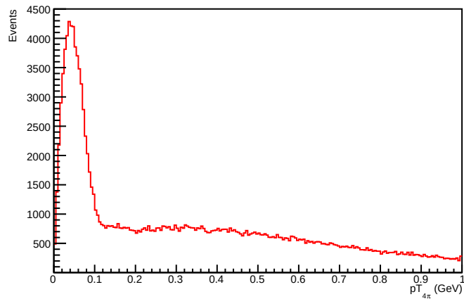
Four-Pion p_T Distribution
