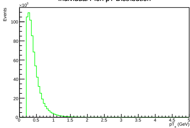
Individual Pion p_T Distribution
