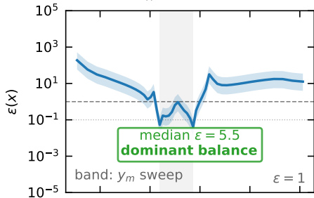
(a) BFS ( Re_H = 13\,700 )
