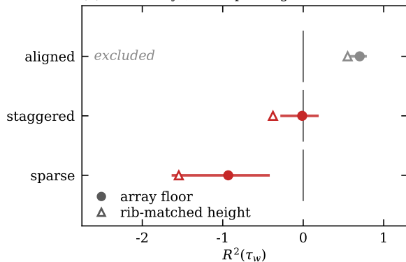
(b) cube arrays, three packings
