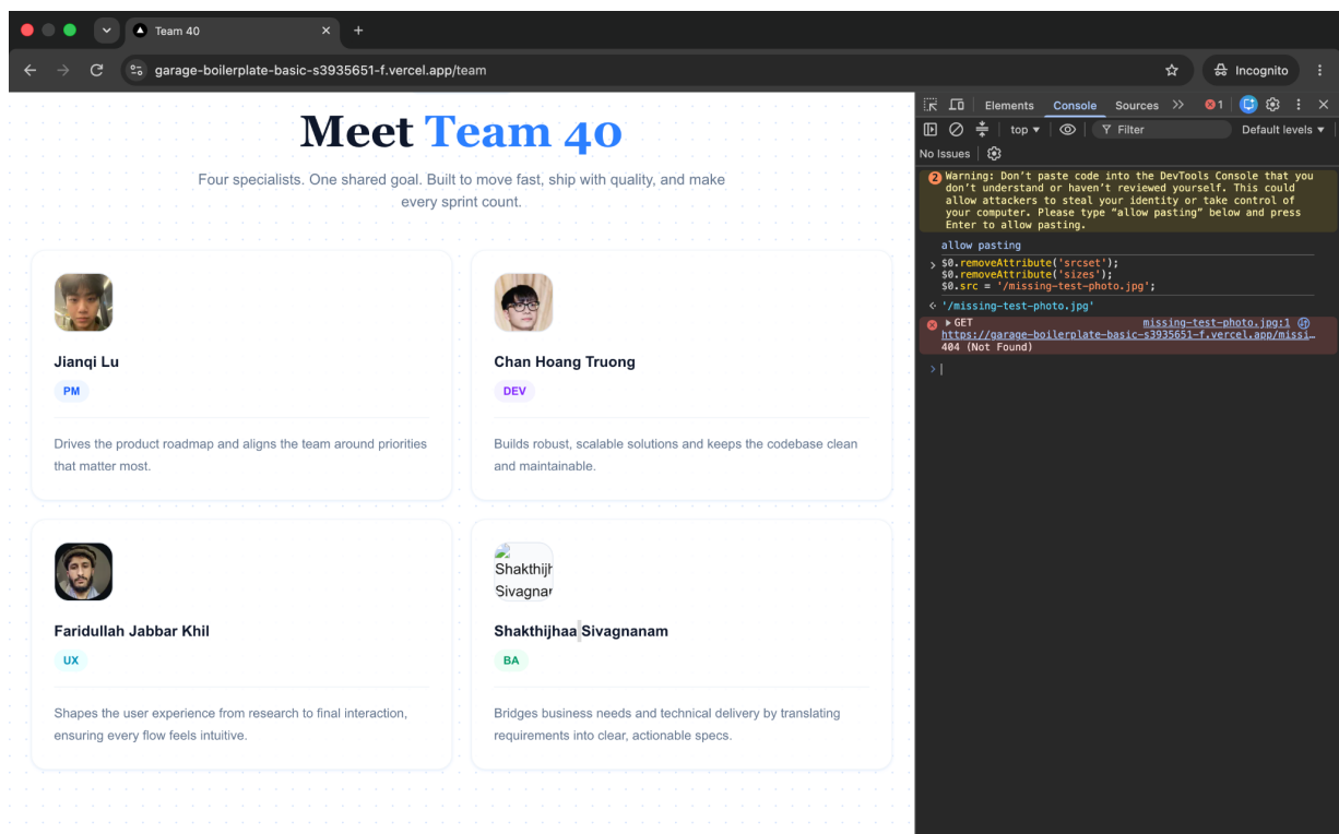
Fig. 3 — Missing-photo edge-case failure. DevTools shows the deliberately invalid image source and a 404 (Not Found) response; the profile card displays a broken image/alt text instead of the required fallback avatar.
