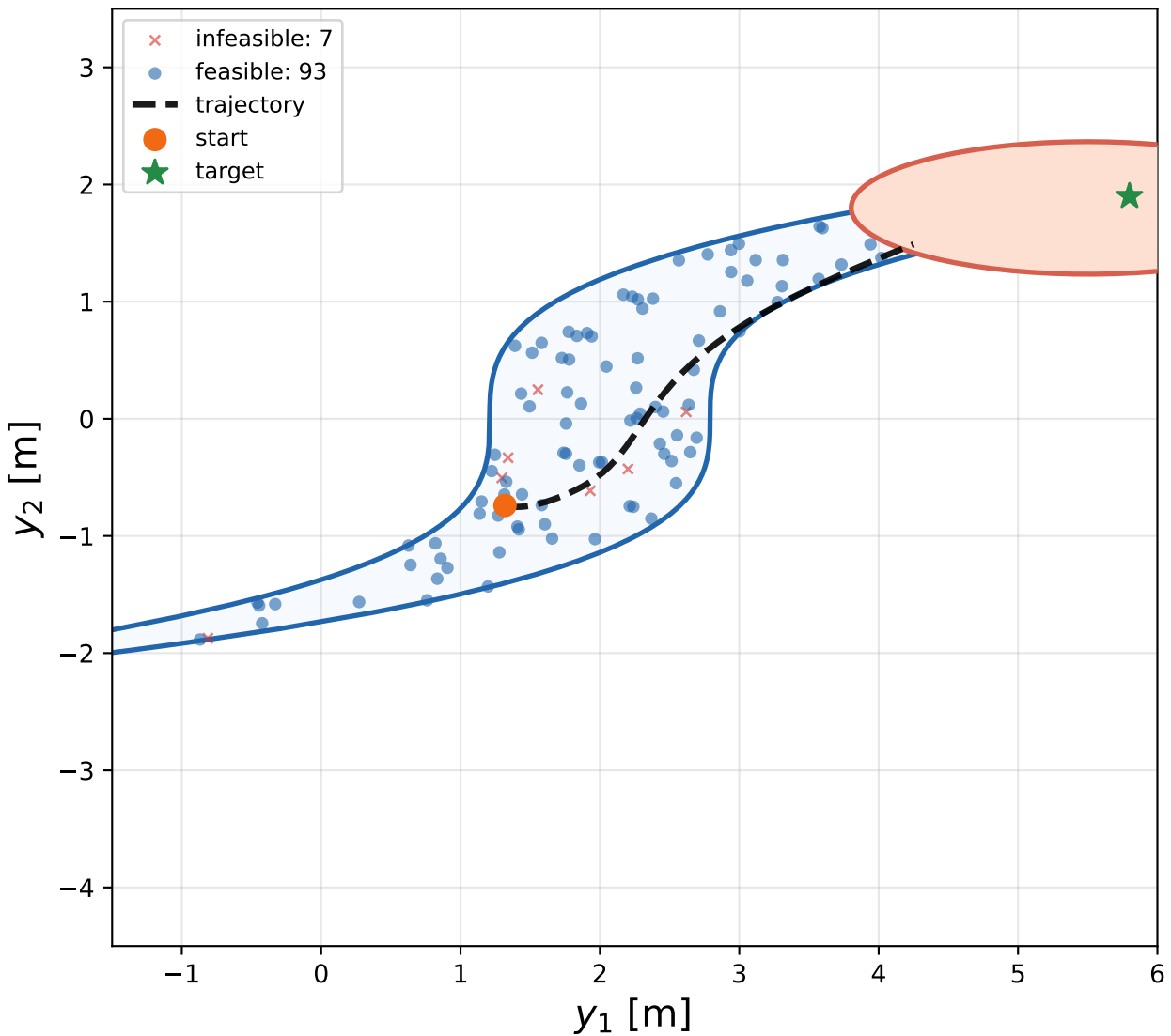
RA-MPC — feasible 93.0% (reaches target)
