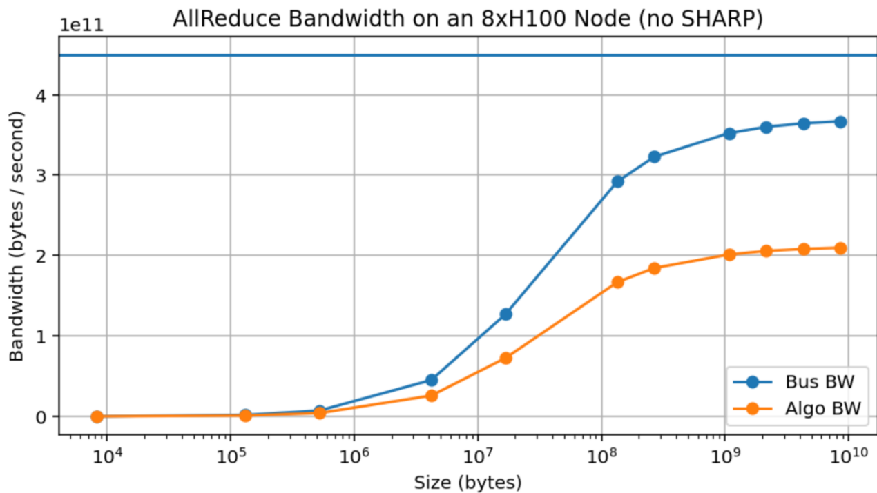
Figure 41: Figure: AllReduce bandwidth on an 8xH100 cluster (intra-node, SHARP disabled).
