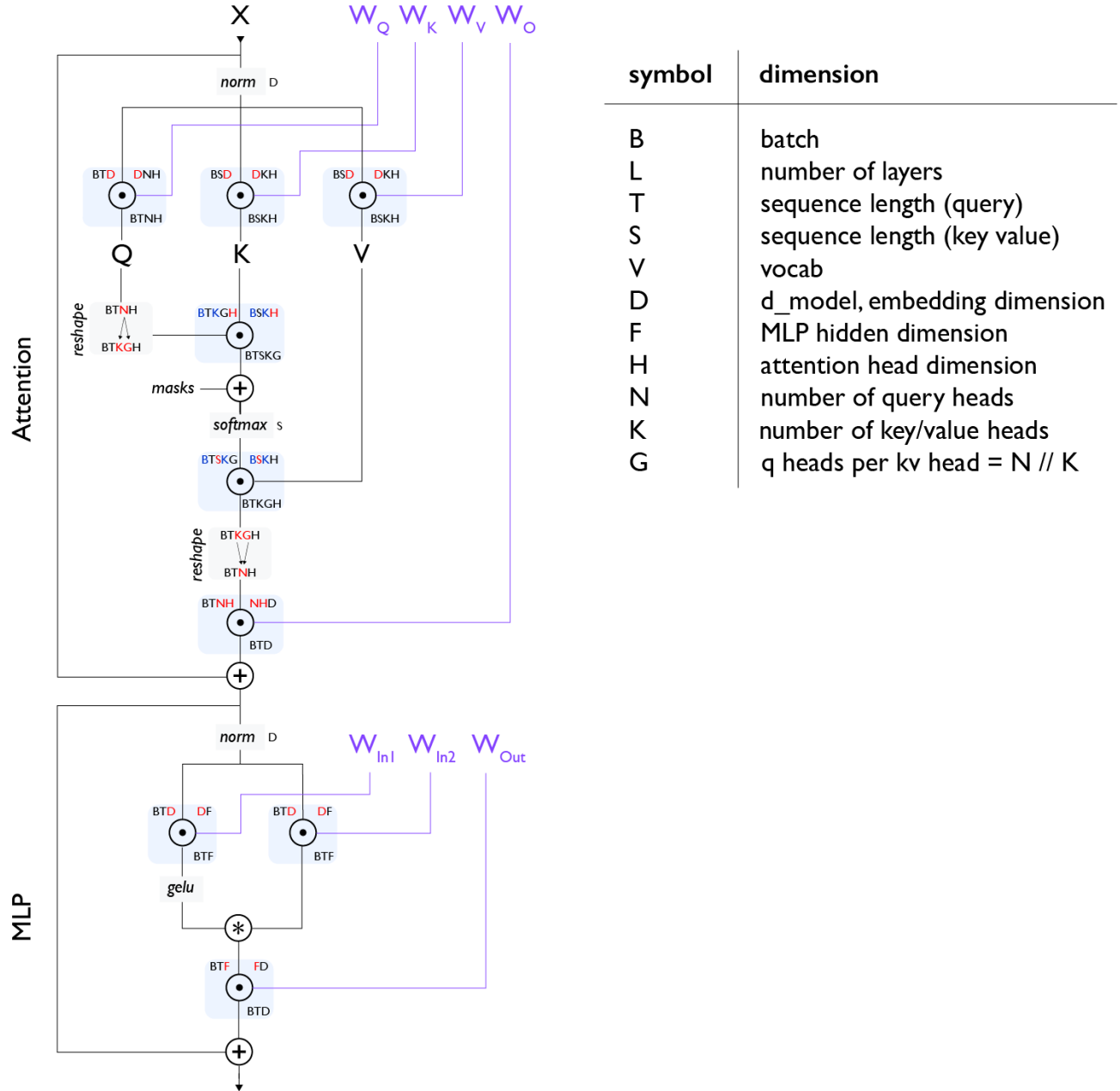
Figure 2: Figure: a standard Transformer layer with each matrix multiplication (matmul) shown as a dot inside a circle. All parameters (excluding norms) are shown in purple. Section 4 walks through this diagram in more detail.
