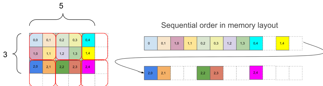
F32[3,5] with tile size of 2x2
