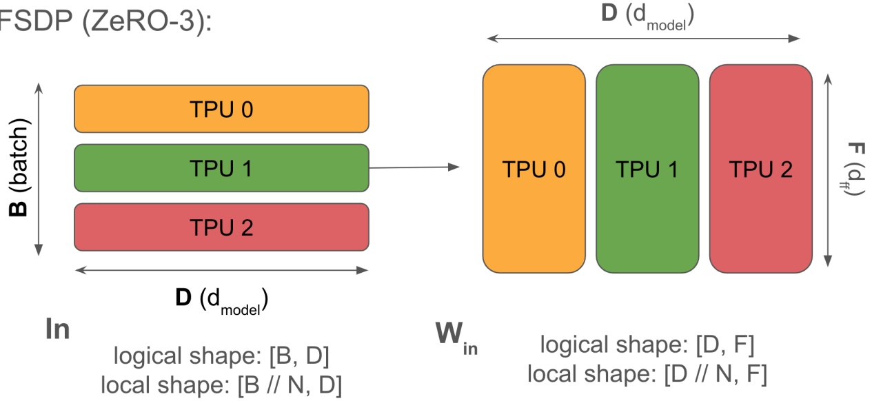
Figure 14: Figure: FSDP shards the contracting dimension of W_{\text{in}} and the output dimension of W_{\text{out}} along the data dimension. This reduces memory but (from Section 3) requires us to gather the weights for W before we perform the matmul. Note that the activations (left) are not sharded along the contracting dimension, which is what forces us to gather. Note that our weight optimizer state is likewise sharded along the contracting dimension.
