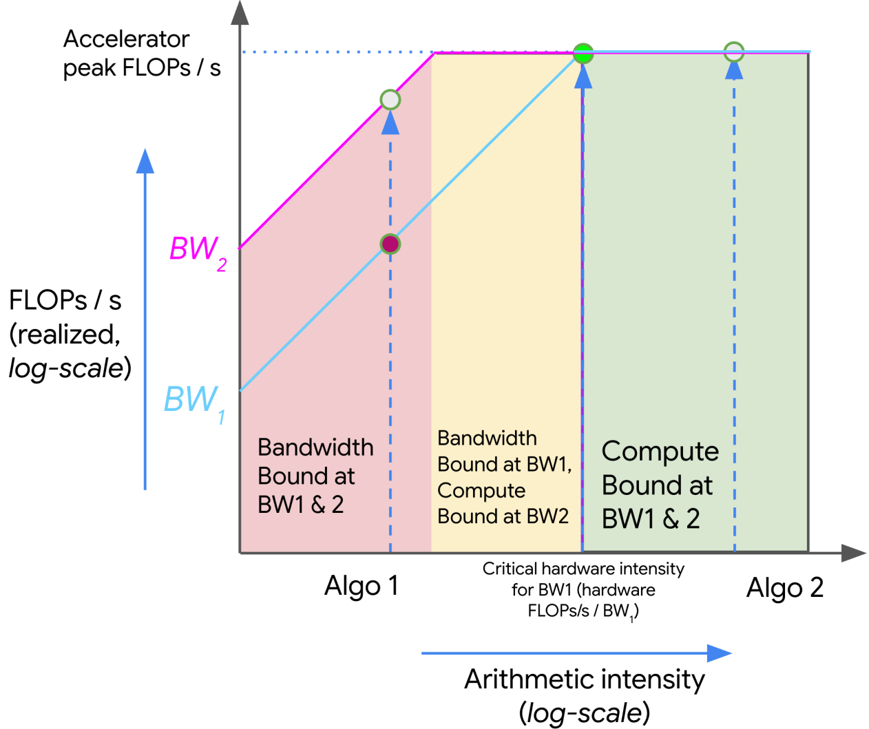
Figure 3: Figure: an example roofline plot showing two algorithms with different arithmetic intensities (Algo 1 and Algo 2) and their corresponding theoretical peak throughput under different bandwidths ( BW_1 and BW_2 ). In the red area, an algorithm is bandwidth bound at both bandwidths and is wasting some fraction of the hardware's peak FLOPs/s. The yellow area is bandwidth-bound only at the lower bandwidth ( BW_1 ). The green area is compute-bound at all bandwidths. Here, we are using the peak FLOPs/s of the accelerator and increasing bandwidth or improving intensity yield no benefit.
