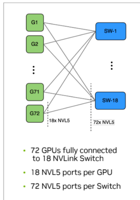
Figure 38: Figure: a diagram showing how a GB200 NVL72 unit is constructed, with 18 switches and 72 GPUs.
