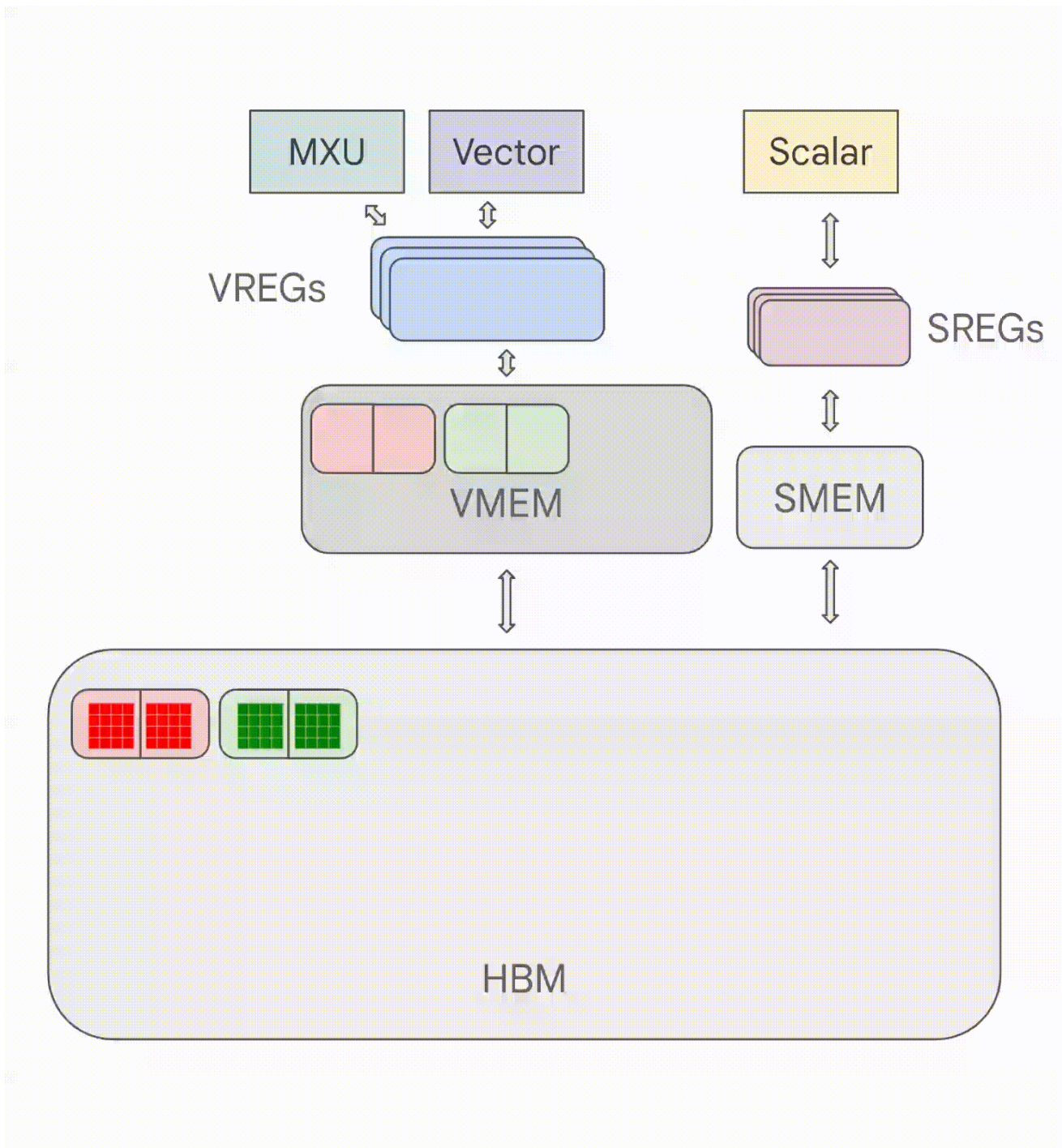
Figure 5: Figure: an animation showing a pointwise product performed on TPU, with bytes loaded from HBM. Note how bytes are streamed out of memory in chunks and partial results are pipelined back without waiting for the full array to be materialized.
