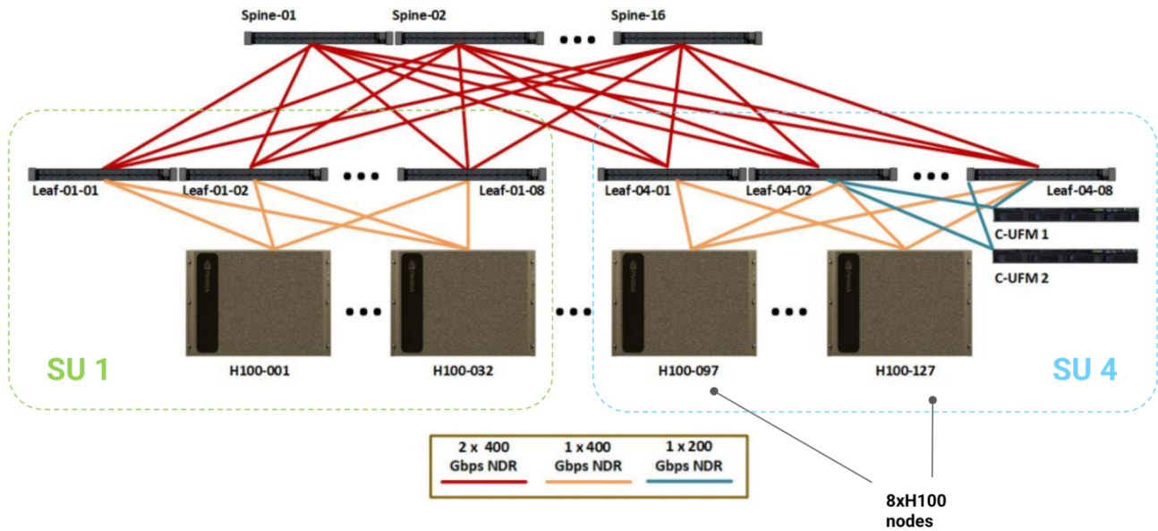
Figure 29: Figure: diagram of the reference 1024 H100 DGX SuperPod with 128 nodes (sometimes 127), each with 8 H100 GPUs, connected to an InfiniBand scale-out network. Sets of 32 nodes (256 GPUs) are called ‘Scalable Units’ or SUs. The leaf and spine IB switches provide enough bandwidth for full bisection bandwidth between nodes.
