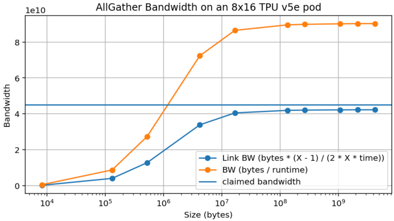
Figure 44: Figure: AllGather bandwidth on a TPU v5e 8x16 cluster (along one axis).
