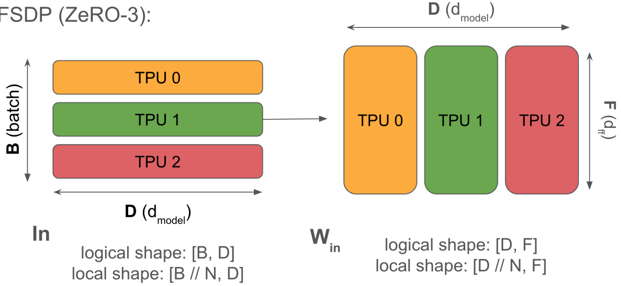
Figure 14: Figure: FSDP shards the contracting dimension of W_{\text{in}} and the output dimension of W_{\text{out}} along the data dimension. This reduces memory but (from Section 3) requires us to gather the weights for W before we perform the matmul. Note that the activations (left) are not sharded along the contracting dimension, which is what forces us to gather. Note that our weight optimizer state is likewise sharded along the contracting dimension.
