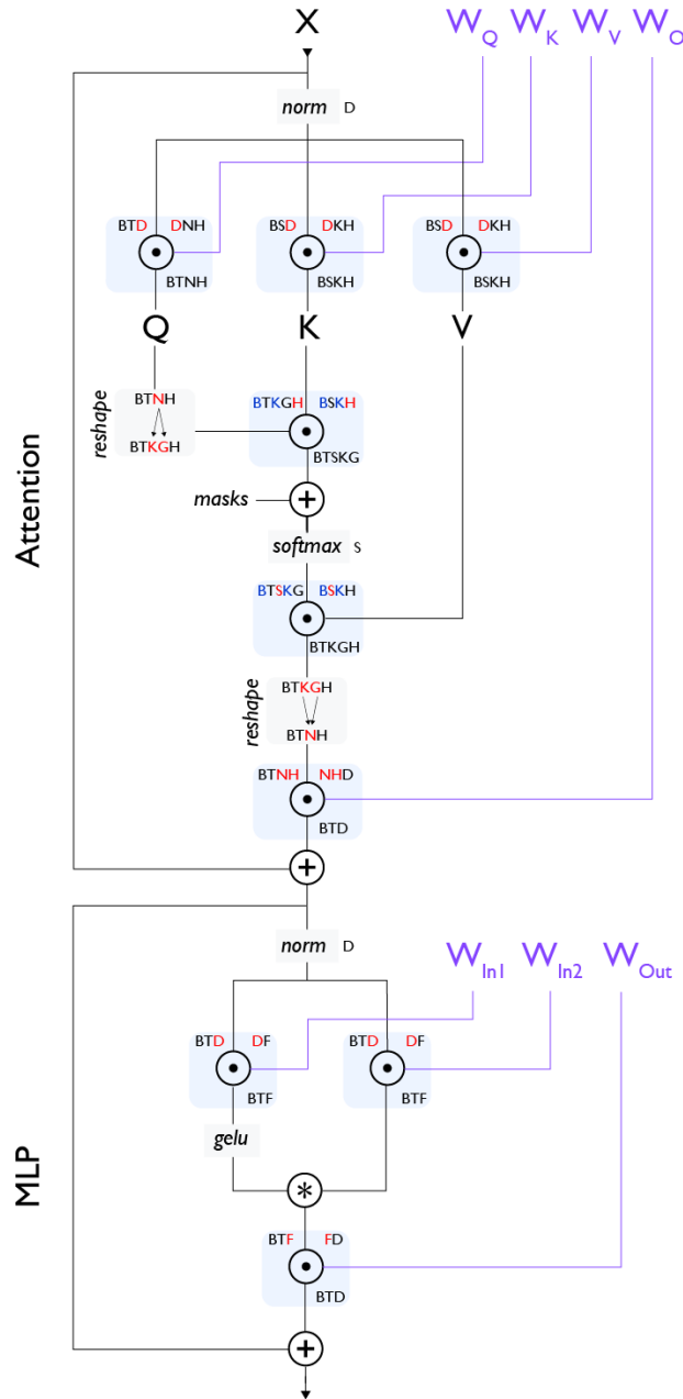
Figure 11: Figure: this diagram shows one layer of a standard Transformer and flows from top-to-bottom. We use a single-letter convention to describe the shapes and layouts of arrays in a Transformer, again showing contracting dimensions in red, and batched dimensions in blue. In a given operation, the input shape is given on top-left and the parameter shape is given on the top-right, with the resulting shape below, e.g. BTD is the input shape for the gating einsum and DF is the weight shape.
