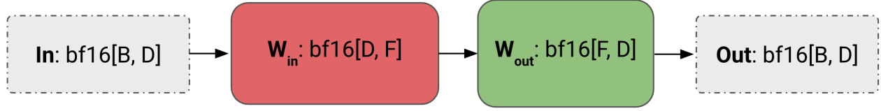
Figure 12: Figure: a simplified Transformer layer. We treat each FFW block as a stack of two matrices W_{in} : bf16[D, F] (up-projection) and W_{out} : bf16[F, D] (down-projection) with an input In : bf16[B, D] .
