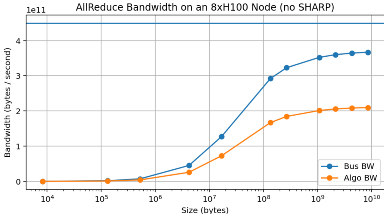
Figure 32: Figure: AllReduce throughput for an 8xH100 node with SHARP disabled. The blue curve is the empirical link bandwidth, calculated as 2 \cdot \text{bytes} \cdot (N - 1) / (N \cdot \text{runtime}) from the empirical measurements. Note that we do not get particularly close to the claimed bandwidth of 450GB/s, even with massive 10GB arrays.
