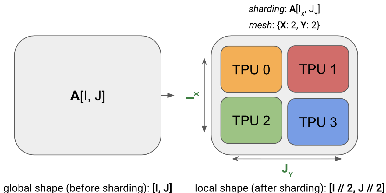
Figure 7: Figure: an example array of shape A[I, J] gets sharded across 4 devices. Both dimensions are evenly sharded across 2 devices with a sharding A[IX, JY] . Each TPU holds 1/4 of the total memory.
