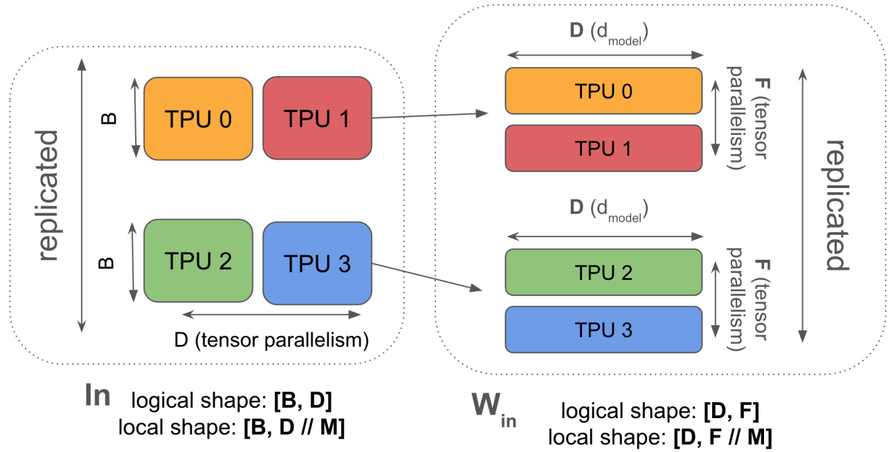
Figure 15: Figure: an example of basic tensor parallelism. Since we're only sharding our activations over Y (unlike in FSDP where we shard over X), we replicate our activations over X. Using our standard syntax, this is A[B, DY] * B[D, FY] \rightarrow C[B, FY] . Because we're only sharding over one of the contracting dimensions, we typically AllGather the activations A before the matmul.
