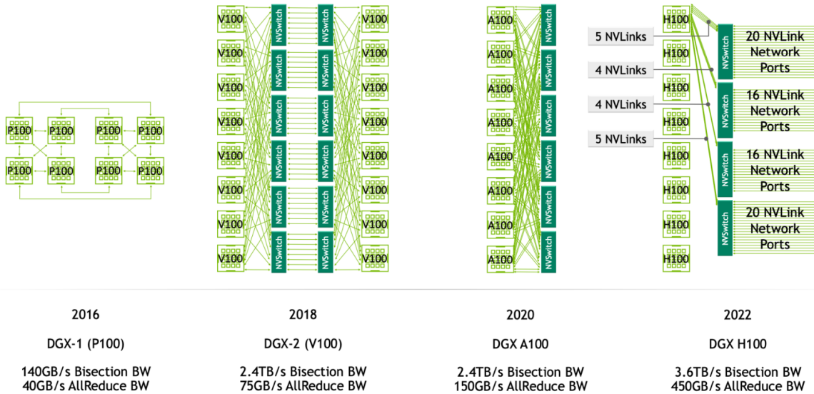
Figure 28: Figure: node aka NVLink domain diagrams from Pascal (P100) onward. Since Volta (V100), we have had all-to-all connectivity within a node using a set of switches. The H100 node has 4 NVSwitches connected to all 8 GPUs with 25GB/s links.
