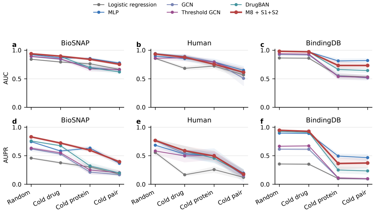
Figure 2: Comparison of feature-only, graph-based, bilinear-attention and full S1/S2 models across the four fixed split scenarios. Each point is the mean of 15 seed-fold evaluations and the shaded band denotes the sample standard deviation.
