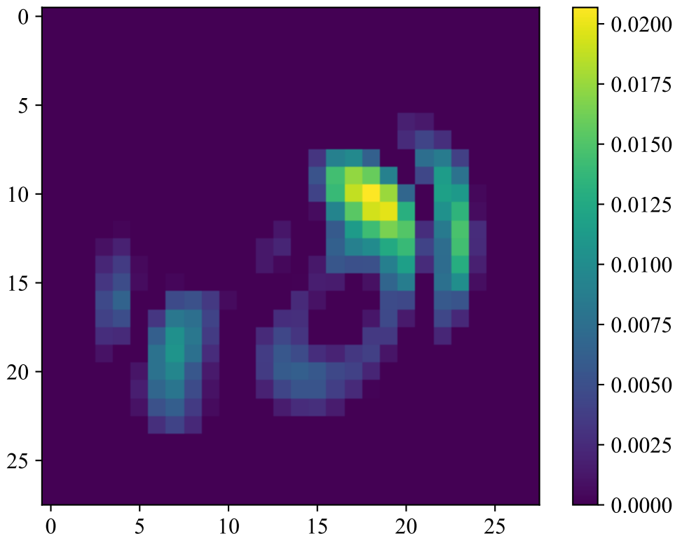
Linear model with 180 features
