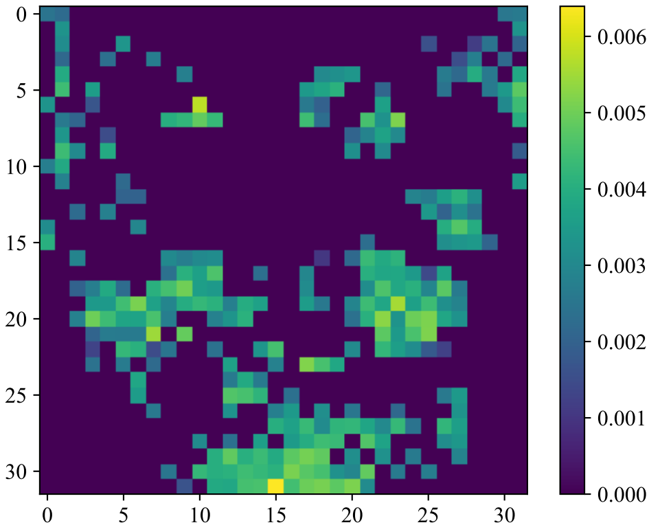
Linear model with 291 features
