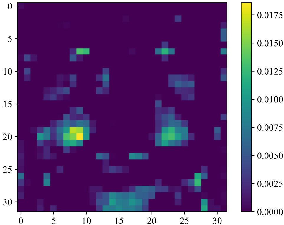
Linear model with 232 features
