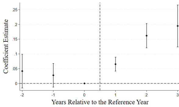
(c) Support Rate
