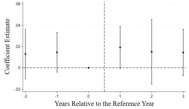
(b) Facility-Level Emission (Balanced)
