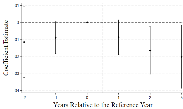
(a) GHG Proposal Dummy
