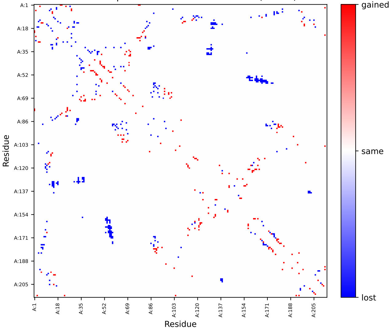
Contact map delta: structure2 - structure1 (< 10 Å)
