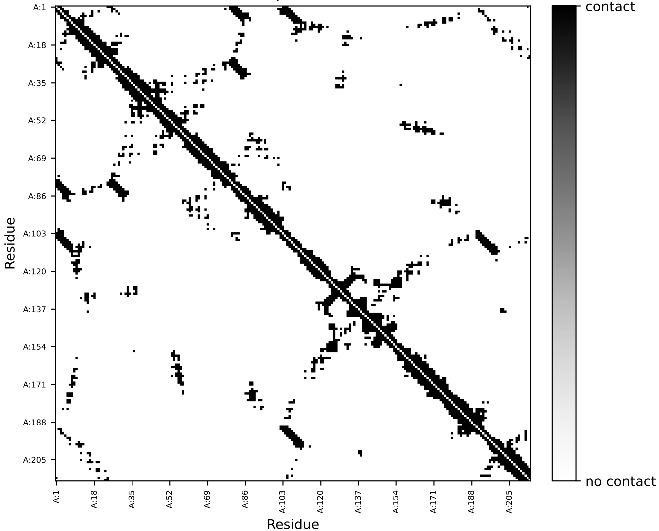
Structure 1 C-alpha contacts < 10 Å
