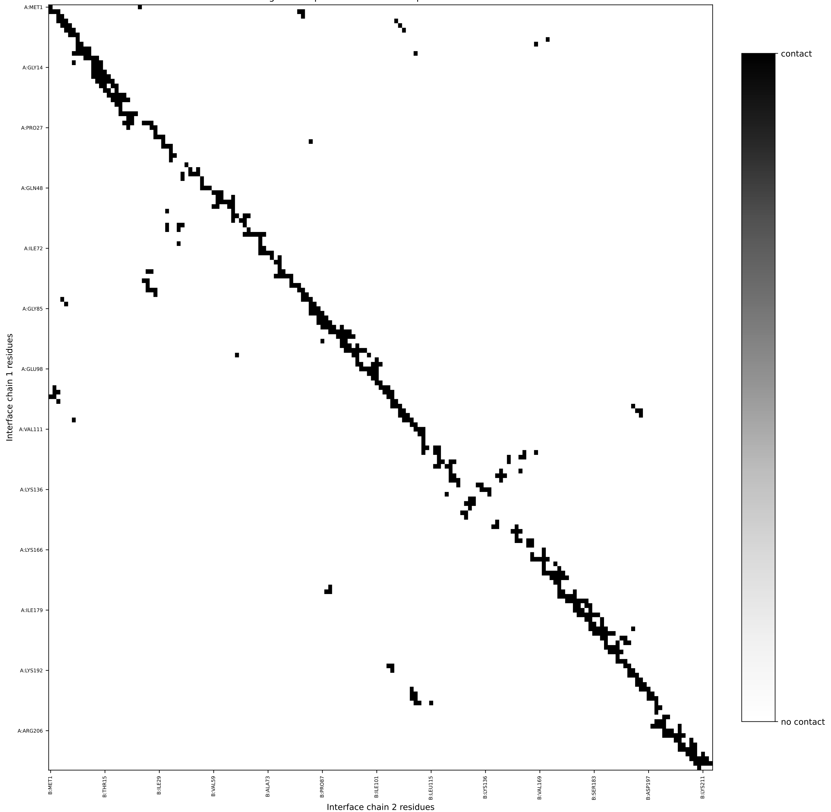
Aligned complex: chain A vs B C-alpha contacts < 5 Å
