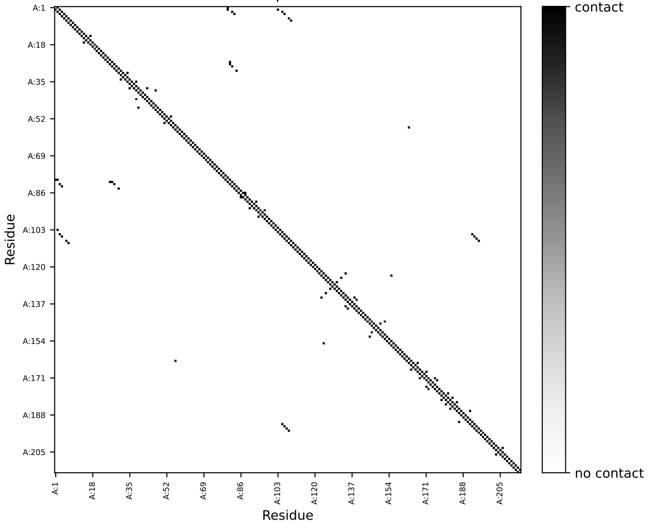
Structure 1 C-alpha contacts < 5 A
