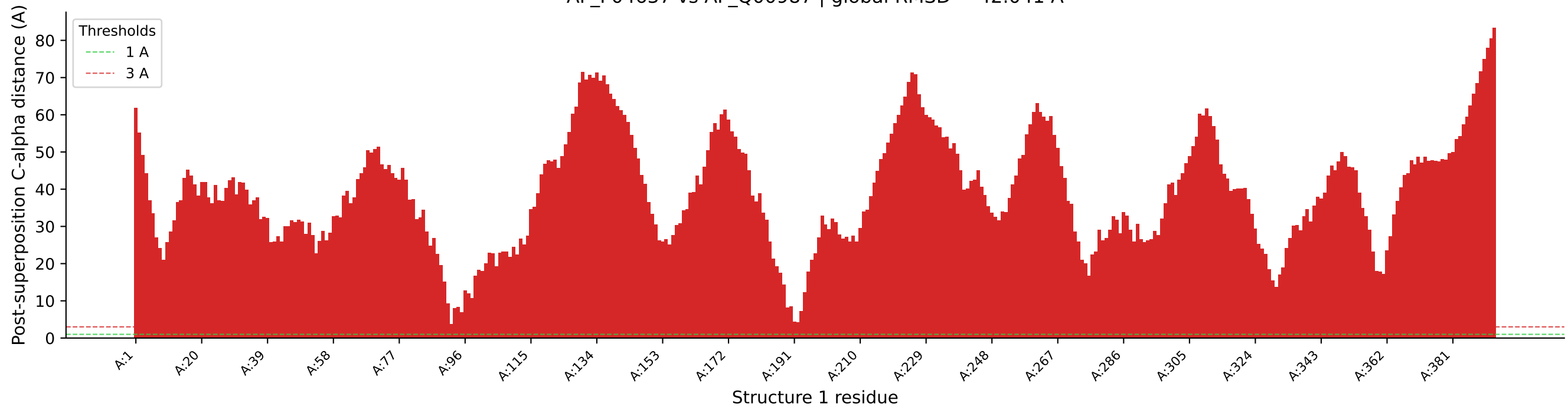
AF_P04637 vs AF_Q00987 | global RMSD = 42.041 A
