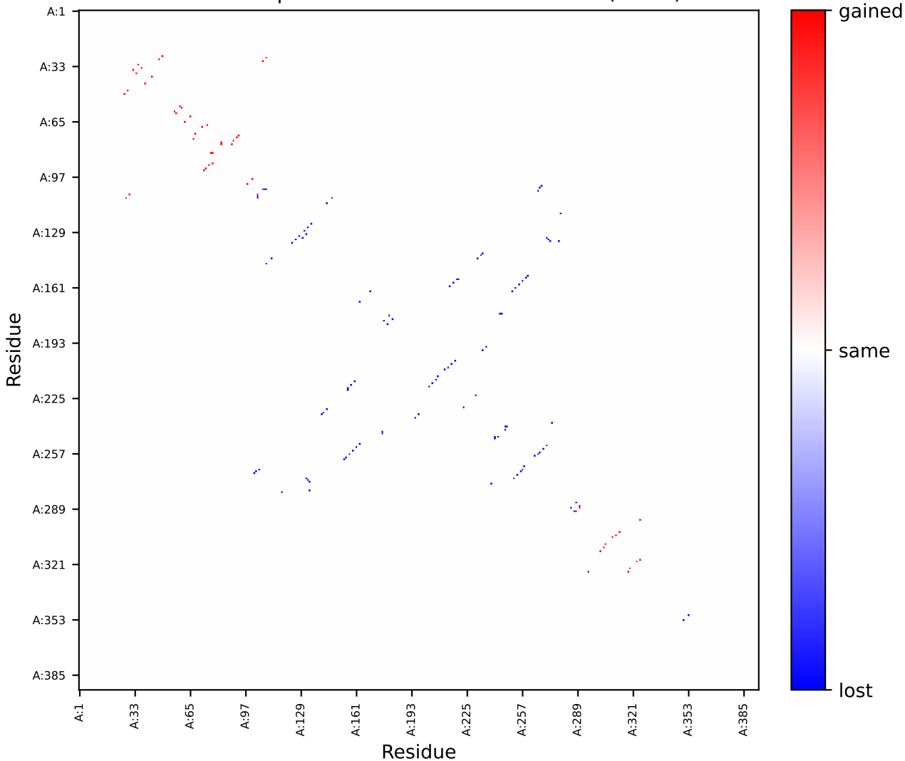
Contact map delta: structure2 - structure1 (< 5 Å)
