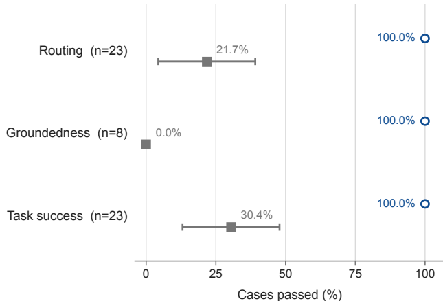
a Strict micro pass rate
