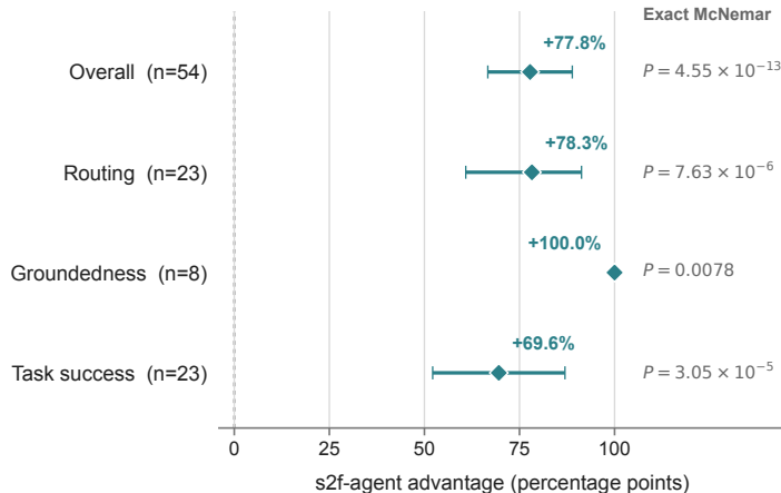
b Paired pass-rate difference
