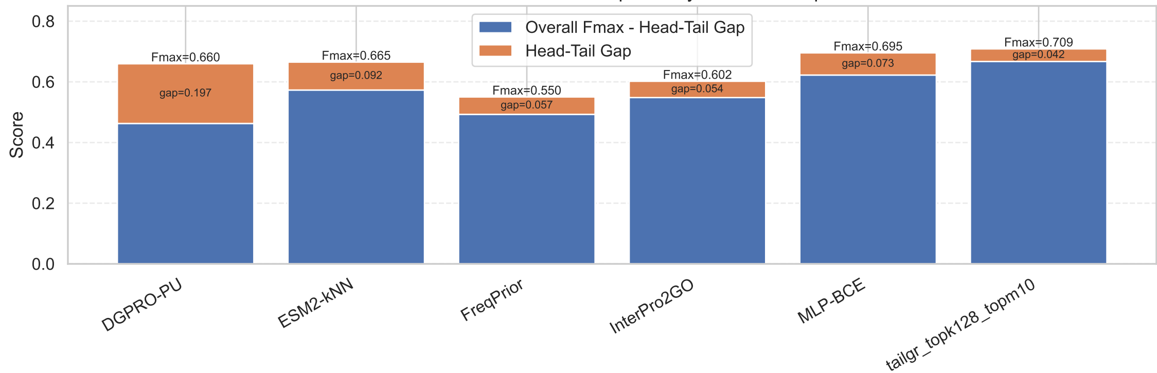
EC: Overall Fmax Decomposed by Head-Tail Gap
