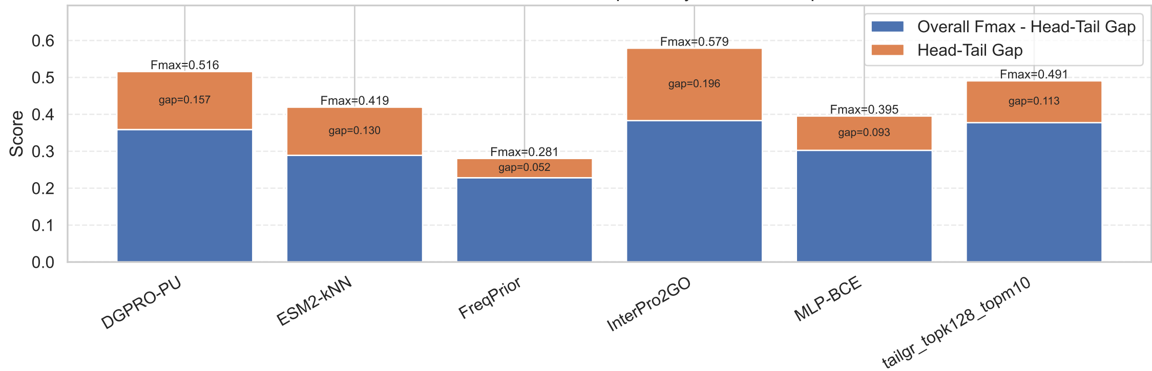
MF: Overall Fmax Decomposed by Head-Tail Gap
