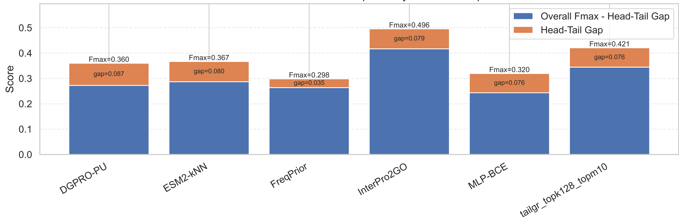
CC: Overall Fmax Decomposed by Head-Tail Gap
