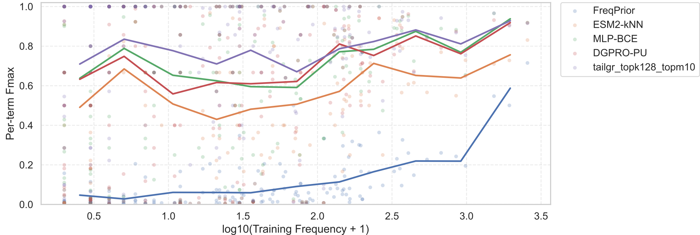
EC: Per-term Fmax vs Training Frequency
