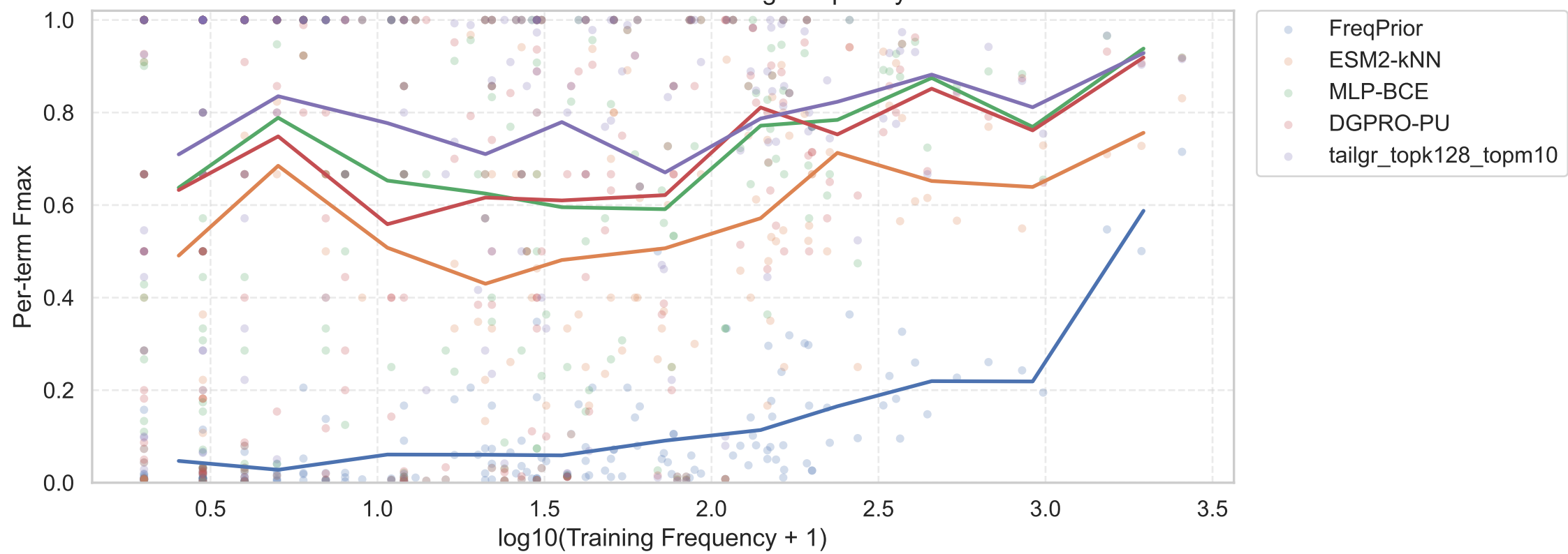
MF: Per-term Fmax vs Training Frequency
