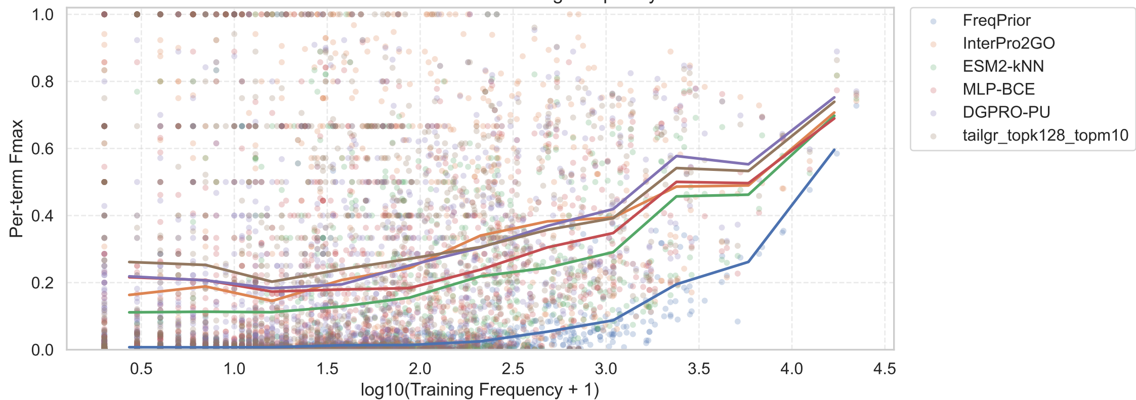
BP: Per-term Fmax vs Training Frequency
