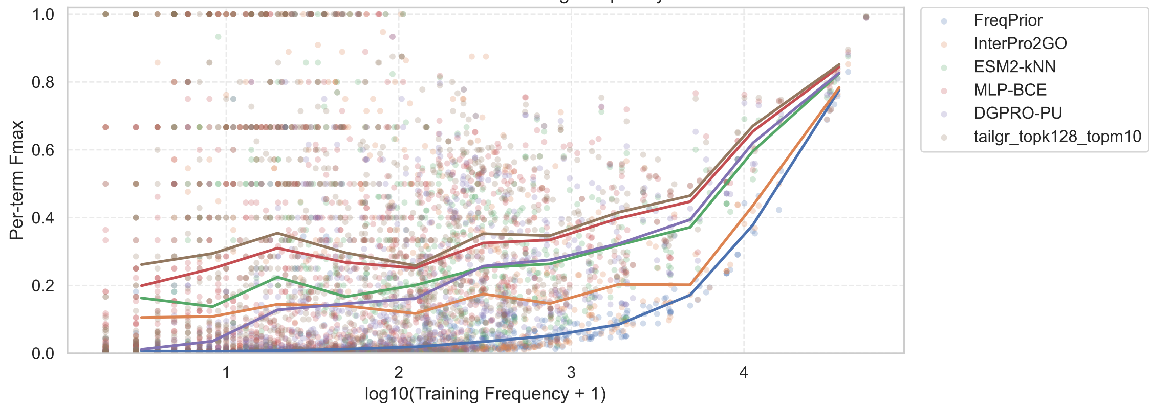
CC: Per-term Fmax vs Training Frequency
