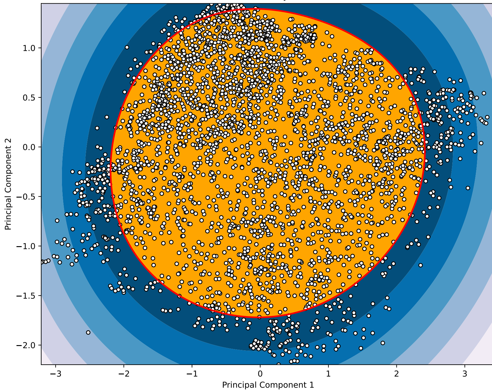
One-Class SVM Decision Boundary on PCA-Transformed Data
