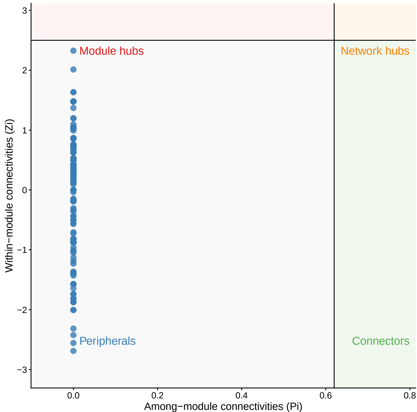
Zi-Pi topological roles
