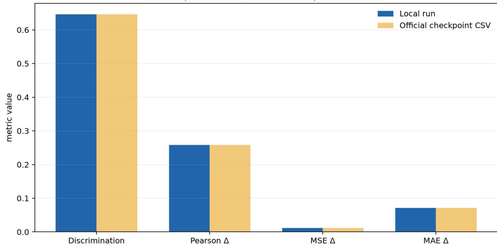
Local reproduction vs official checkpoint reference
